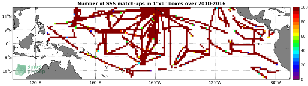
Figure 4: Number of SSS match-ups between TSG-SAMOS SSS and the SMOS-L3-ICDC-V3-MONTHLY-0.5DEG SSS product for the Tropical Pacific Ocean Pi-MEP region over 1^\circ \times 1^\circ boxes and for the full satellite product period.
