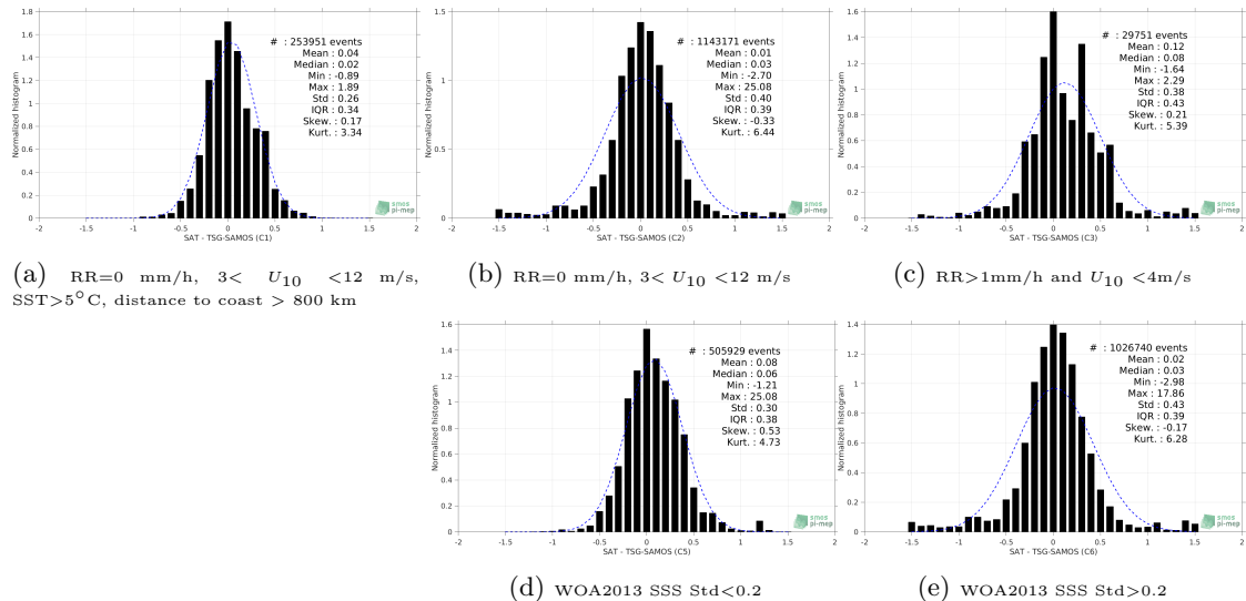
Figure 13: Normalized histogram of \Delta SSS (SMOS-L3-ICDC-V3-MONTHLY-0.5DEG - TSG-SAMOS) for 5 different subdatasets corresponding to: RR=0 mm/h, 3 < U_{10} < 12 m/s, SST >5^\circ\text{C} , distance to coast > 800 km (a), RR=0 mm/h, 3 < U_{10} < 12 m/s (b), RR >1 mm/h and U_{10} < 4 m/s (c), WOA2013 SSS Std <0.2 (d), WOA2013 SSS Std >0.2 (e).
