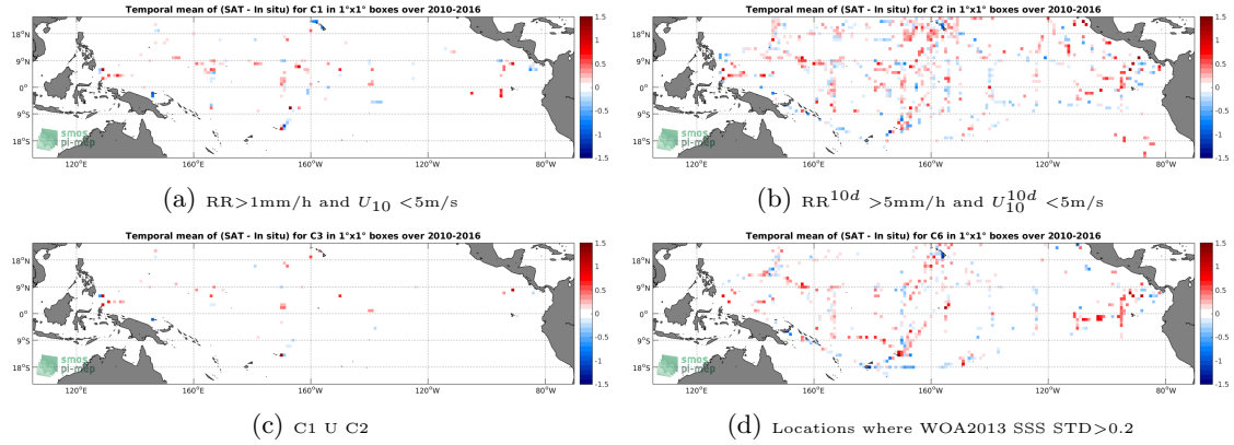
Figure 12: Temporal mean gridded over spatial boxes of size 1^\circ \times 1^\circ of \Delta SSS (SMOS-L3-ICDC-V3-MONTHLY-0.5DEG - TSG-SAMOS) for 4 different subdatasets corresponding to: RR > 1mm/h and U_{10} < 5\text{m/s} (a), RR^{10d} > 5\text{mm/h} and U_{10}^{10d} < 5\text{m/s} (b), C1 U C2 (c), Locations where WOA2013 SSS STD > 0.2 (d).
