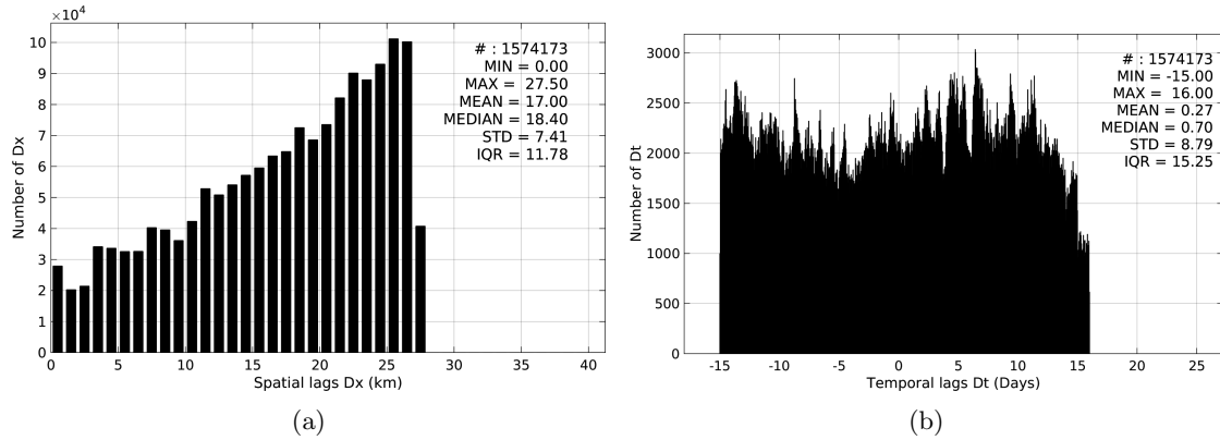
Figure 5: Histograms of the spatial (a) and temporal (b) lags between the time of the TSG-SAMOS measurements and the date of the corresponding SMOS-L3-ICDC-V3-MONTHLY-0.5DEG SSS product.
