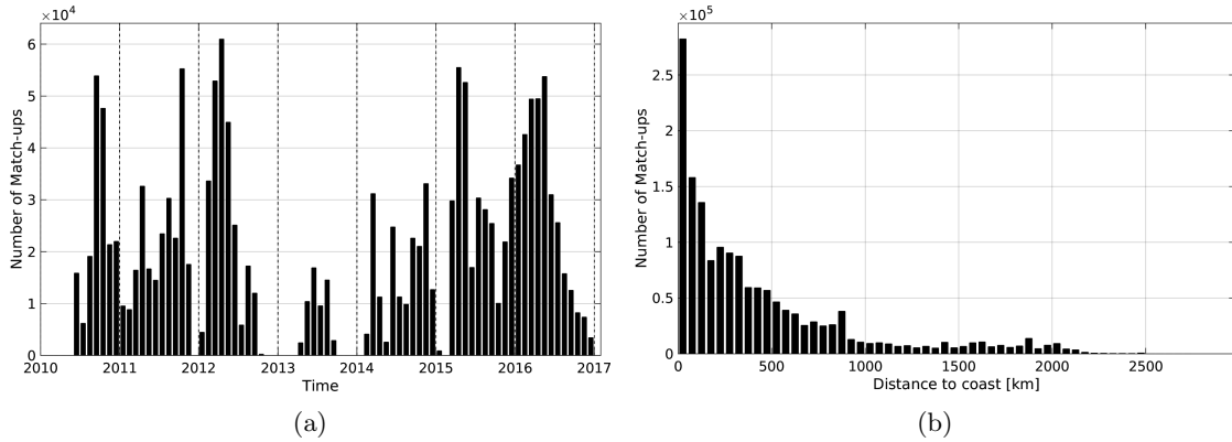
Figure 1: Number of match-ups between TSG-SAMOS and SMOS-L3-ICDC-V3-MONTHLY-0.5DEG SSS as a function of time (a) and as function of the distance to coast (b) over the Tropical Pacific Ocean Pi-MEP region and for the full satellite product period.
