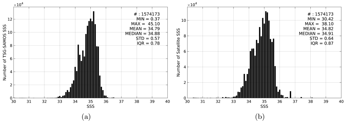
Figure 2: Histograms of SSS from TSG-SAMOS (a) and SMOS-L3-ICDC-V3-MONTHLY-0.5DEG (b) considering all match-up pairs per bins of 0.1 over the Tropical Pacific Ocean Pi-MEP region and for the full satellite product period.
