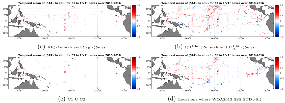
Figure 12: Temporal mean gridded over spatial boxes of size 1^\circ \times 1^\circ of \Delta SSS (SMOS-L3-ICDC-V3-MONTHLY-0.5DEG - TSG-SAMOS) for 4 different subdatasets corresponding to:RR>1mm/h and U_{10} < 5 m/s (a), RR^{10d} > 5 mm/h and U_{10}^{10d} < 5 m/s (b), C1 U C2 (c),Locations where WOA2013 SSS STD>0.2 (d).
