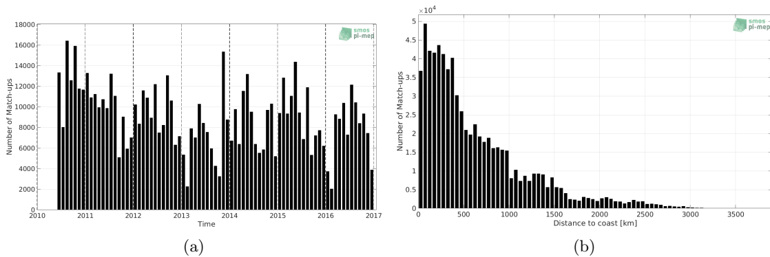
Figure 1: Number of match-ups between TSG (LEGOS-DM) and SMOS SSS L3 v3 Monthly (ICDC) SSS as a function of time (a) and as function of the distance to coast (b) over the Tropical Pacific Ocean Pi-MEP region and for the full satellite product period.
