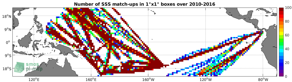
Figure 4: Number of SSS match-ups between TSG (LEGOS-DM) SSS and the SMOS SSS L3 v3 Monthly (ICDC) SSS product for the Tropical Pacific Ocean Pi-MEP region over 1^\circ \times 1^\circ boxes and for the full satellite product period.
