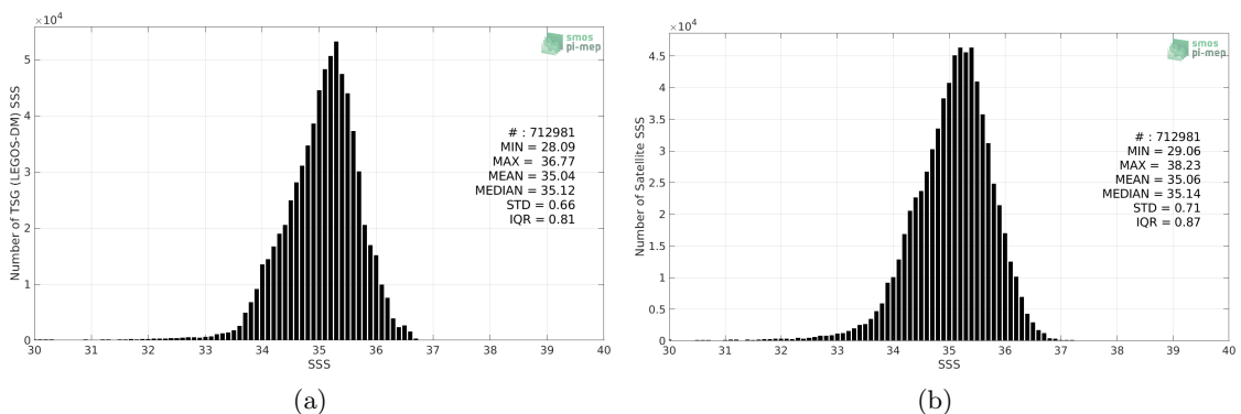
Figure 2: Histograms of SSS from TSG (LEGOS-DM) (a) and SMOS SSS L3 v3 Monthly (ICDC) (b) considering all match-up pairs per bins of 0.1 over the Tropical Pacific Ocean Pi-MEP region and for the full satellite product period.
