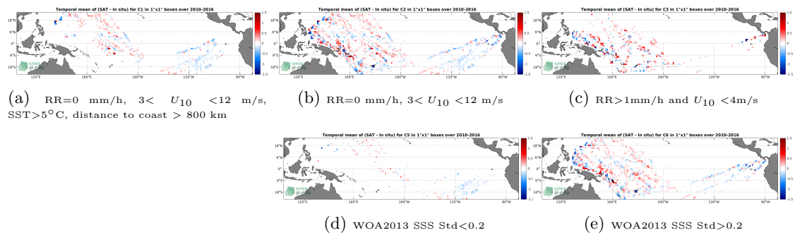
Figure 12: Temporal mean gridded over spatial boxes of size 1^\circ \times 1^\circ of \Delta SSS (SMOS SSS L3 v3 Monthly (ICDC) - TSG (LEGOS-DM)) for 5 different subdatasets corresponding to:RR=0 mm/h, 3 < U_{10} < 12 m/s, SST >5^\circ C, distance to coast > 800 km (a), RR=0 mm/h, 3 < U_{10} < 12 m/s (b), RR >1 mm/h and U_{10} < 4 m/s (c), WOA2013 SSS Std <0.2 (d), WOA2013 SSS Std >0.2 (e).
