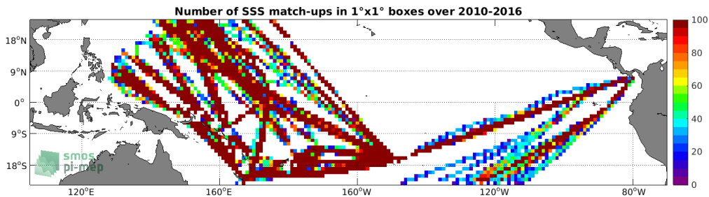
Figure 4: Number of SSS match-ups between TSG (LEGOS-DM) SSS and the SMOS SSS L3 v3 Monthly (ICDC) SSS product for the Tropical Pacific Ocean Pi-MEP region over 1^\circ \times 1^\circ boxes and for the full satellite product period.
