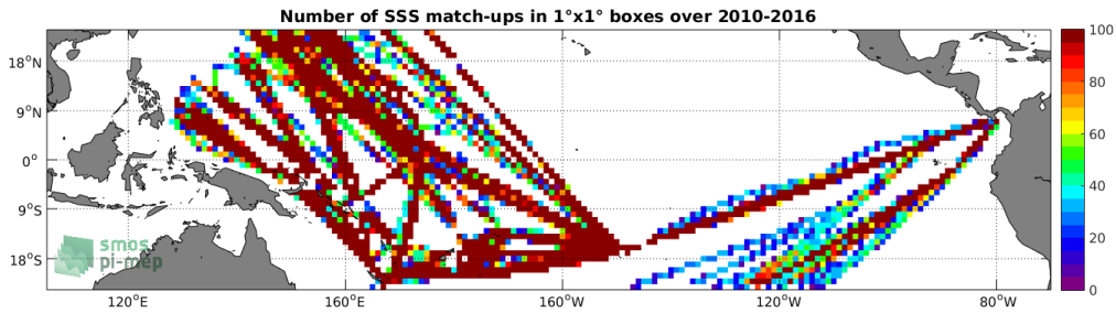
Figure 4: Number of SSS match-ups between TSG-LEGOS-DM SSS and the SMOS-L3-ICDC-V3-MONTHLY-0.5DEG SSS product for the Tropical Pacific Ocean Pi-MEP region over 1°x1° boxes and for the full satellite product period.
