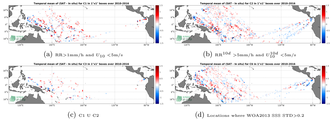
Figure 12: Temporal mean gridded over spatial boxes of size 1^\circ \times 1^\circ of \Delta SSS (SMOS-L3-ICDC-V3-MONTHLY-0.5DEG - TSG-LEGOS-DM) for 4 different subdatasets corresponding to: RR > 1\text{mm/h} and U_{10} < 5\text{m/s} (a), RR^{10d} > 5\text{mm/h} and U_{10}^{10d} < 5\text{m/s} (b), C1 U C2 (c), Locations where WOA2013 SSS STD > 0.2 (d).
