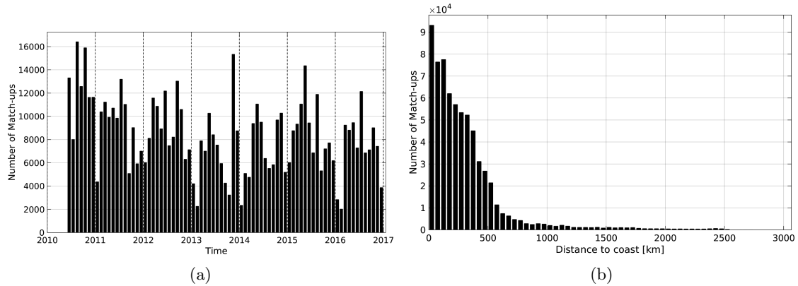
Figure 1: Number of match-ups between TSG-LEGOS-DM and SMOS-L3-ICDC-V3-MONTHLY-0.5DEG SSS as a function of time (a) and as function of the distance to coast (b) over the Tropical Pacific Ocean Pi-MEP region and for the full satellite product period.
