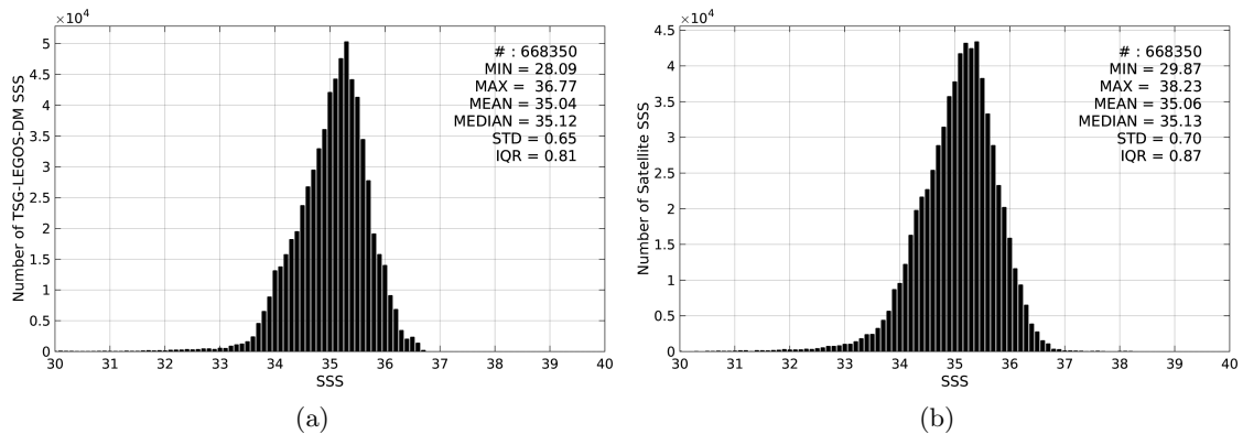
Figure 2: Histograms of SSS from TSG-LEGOS-DM (a) and SMOS-L3-ICDC-V3-MONTHLY-0.5DEG (b) considering all match-up pairs per bins of 0.1 over the Tropical Pacific Ocean Pi-MEP region and for the full satellite product period.
