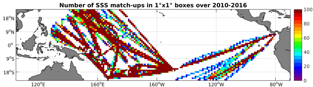
Figure 4: Number of SSS match-ups between TSG-LEGOS-DM SSS and the SMOS-L3-ICDC-V3-MONTHLY-0.5DEG SSS product for the Tropical Pacific Ocean Pi-MEP region over 1°x1° boxes and for the full satellite product period.
