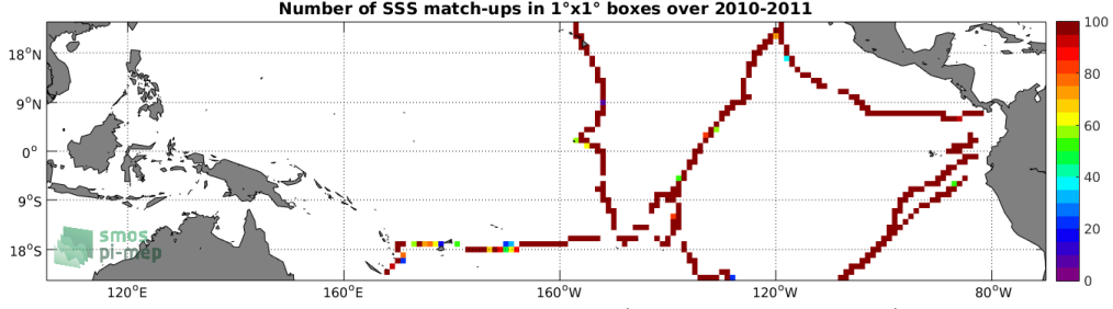
Figure 4: Number of SSS match-ups between TSG (GOSUD-Sailing-ship) SSS and the SMOS SSS L3 v3 Monthly (ICDC) SSS product for the Tropical Pacific Ocean Pi-MEP region over 1^\circ \times 1^\circ boxes and for the full satellite product period.
