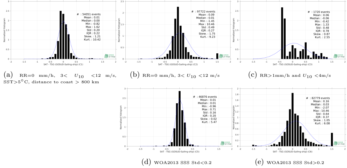
Figure 13: Normalized histogram of \Delta SSS (SMOS SSS L3 v3 Monthly (ICDC) - TSG (GOSUD-Sailing-ship)) for 5 different subdatasets corresponding to: RR=0 mm/h, 3 < U_{10} < 12 m/s, SST>5°C, distance to coast > 800 km (a), RR=0 mm/h, 3 < U_{10} < 12 m/s (b), RR>1mm/h and U_{10} < 4 m/s (c), WOA2013 SSS Std<0.2 (d), WOA2013 SSS Std>0.2 (e).
