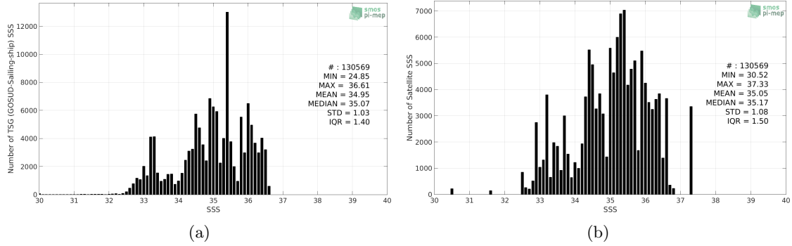
Figure 2: Histograms of SSS from TSG (GOSUD-Sailing-ship) (a) and SMOS SSS L3 v3 Monthly (ICDC) (b) considering all match-up pairs per bins of 0.1 over the Tropical Pacific Ocean Pi-MEP region and for the full satellite product period.
