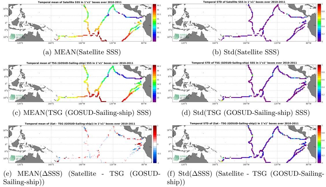
Figure 6: Temporal mean (left) and Std (right) of SSS from SMOS SSS L3 v3 Monthly (ICDC) (top), TSG (GOSUD-Sailing-ship) (middle), and of \Delta SSS (Satellite - TSG (GOSUD-Sailing-ship)). Only match-up pairs are used to generate these maps.
