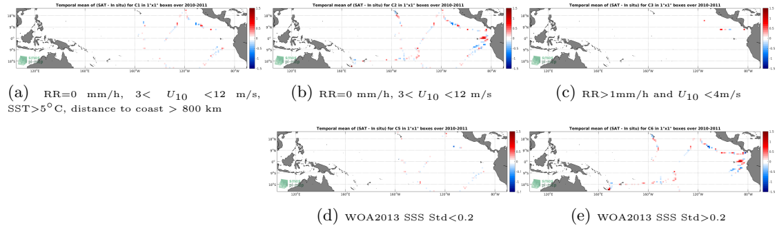
Figure 12: Temporal mean gridded over spatial boxes of size 1^\circ \times 1^\circ of \Delta SSS (SMOS SSS L3 v3 Monthly (ICDC) - TSG (GOSUD-Sailing-ship)) for 5 different subdatasets corresponding to: RR=0 mm/h, 3 < U_{10} < 12 m/s, SST > 5^\circ C , distance to coast > 800 km (a), RR=0 mm/h, 3 < U_{10} < 12 m/s (b), RR > 1 mm/h and U_{10} < 4 m/s (c), WOA2013 SSS Std < 0.2 (d), WOA2013 SSS Std > 0.2 (e).
