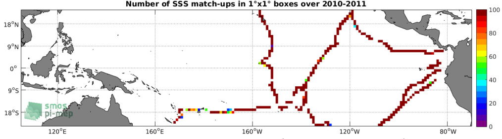
Figure 4: Number of SSS match-ups between TSG (GOSUD-Sailing-ship) SSS and the SMOS SSS L3 v3 Monthly (ICDC) SSS product for the Tropical Pacific Ocean Pi-MEP region over 1°x1° boxes and for the full satellite product period.
