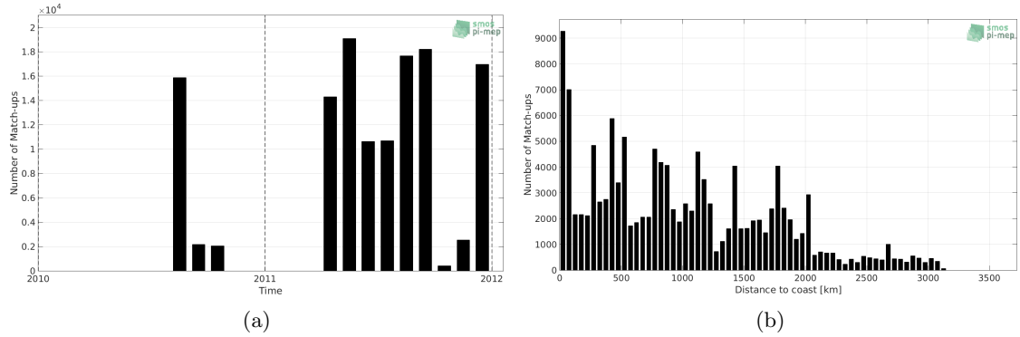
Figure 1: Number of match-ups between TSG (GOSUD-Sailing-ship) and SMOS SSS L3 v3 Monthly (ICDC) SSS as a function of time (a) and as function of the distance to coast (b) over the Tropical Pacific Ocean Pi-MEP region and for the full satellite product period.
