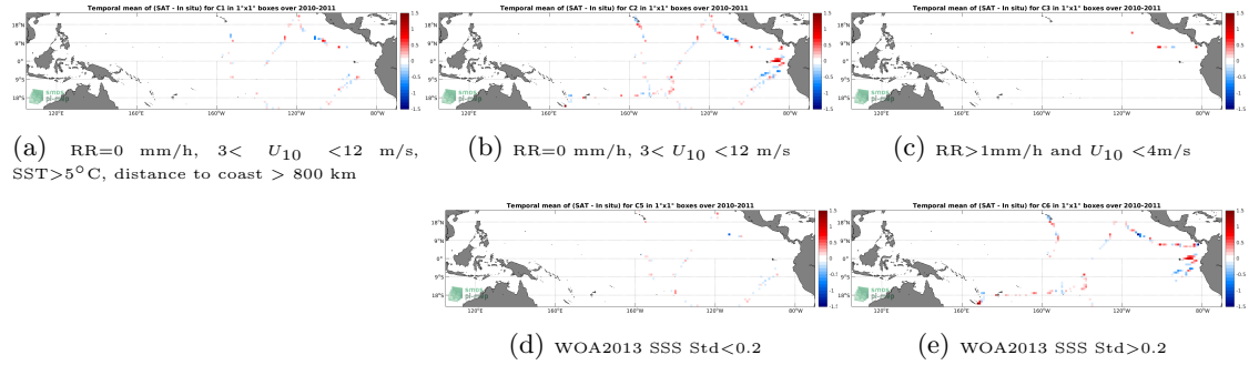
Figure 12: Temporal mean gridded over spatial boxes of size 1^\circ \times 1^\circ of \Delta SSS (SMOS SSS L3 v3 Monthly (ICDC) - TSG (GOSUD-Sailing-ship)) for 5 different subdatasets corresponding to: RR=0 mm/h, 3 < U_{10} < 12 m/s, SST > 5^\circ\text{C} , distance to coast > 800 km (a), RR=0 mm/h, 3 < U_{10} < 12 m/s (b), RR > 1\text{mm/h} and U_{10} < 4\text{m/s} (c), WOA2013 SSS Std < 0.2 (d), WOA2013 SSS Std > 0.2 (e).
