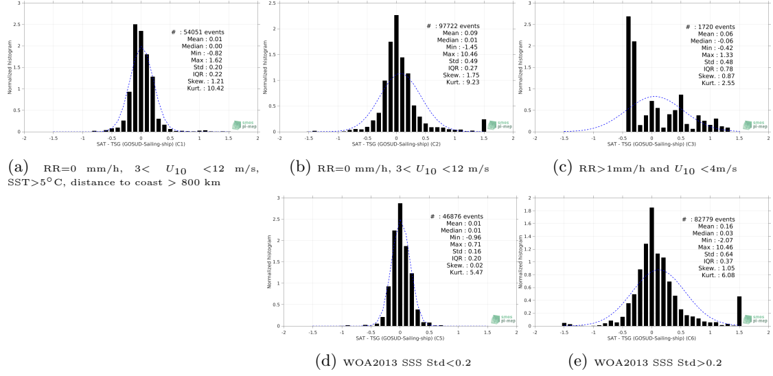
Figure 13: Normalized histogram of \Delta\text{SSS} (SMOS SSS L3 v3 Monthly (ICDC) - TSG (GOSUD-Sailing-ship)) for 5 different subdatasets corresponding to: RR=0 mm/h, 3 < U_{10} < 12 m/s, SST > 5^\circ\text{C} , distance to coast > 800 km (a), RR=0 mm/h, 3 < U_{10} < 12 m/s (b), RR > 1 mm/h and U_{10} < 4 m/s (c), WOA2013 SSS Std < 0.2 (d), WOA2013 SSS Std > 0.2 (e).
