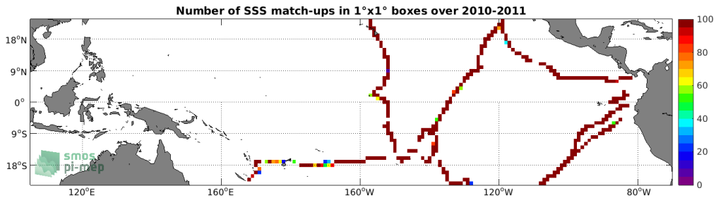
Figure 4: Number of SSS match-ups between TSG (GOSUD-Sailing-ship) SSS and the SMOS SSS L3 v3 Monthly (ICDC) SSS product for the Tropical Pacific Ocean Pi-MEP region over 1^\circ \times 1^\circ boxes and for the full satellite product period.
