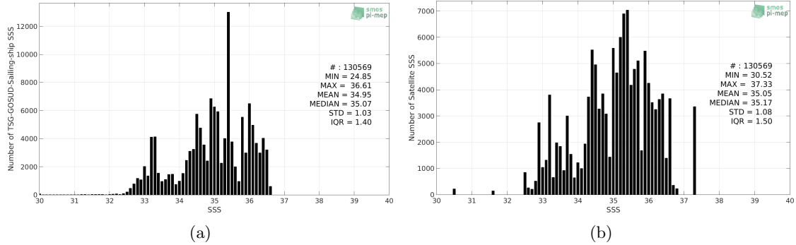
Figure 2: Histograms of SSS from TSG-GOSUD-Sailing-ship (a) and SMOS-L3-ICDC-V3-MONTHLY-0.5DEG (b) considering all match-up pairs per bins of 0.1 over the Tropical Pacific Ocean Pi-MEP region and for the full satellite product period.
