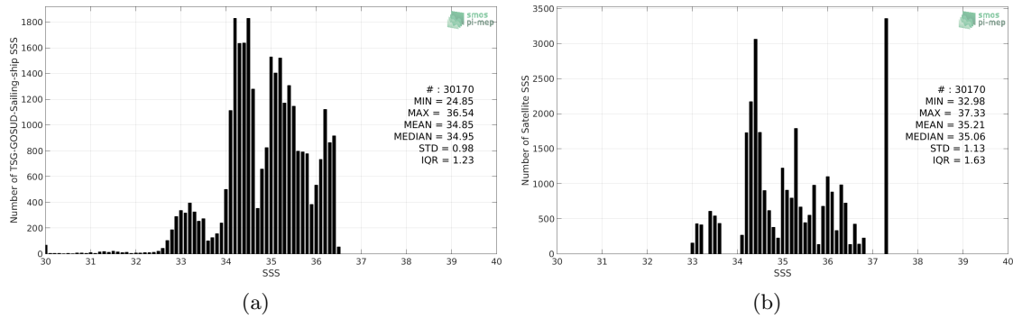
Figure 2: Histograms of SSS from TSG-GOSUD-Sailing-ship (a) and SMOS-L3-ICDC-V3-MONTHLY-0.5DEG (b) considering all match-up pairs per bins of 0.1 over the Tropical Pacific Ocean Pi-MEP region and for the full satellite product period.
