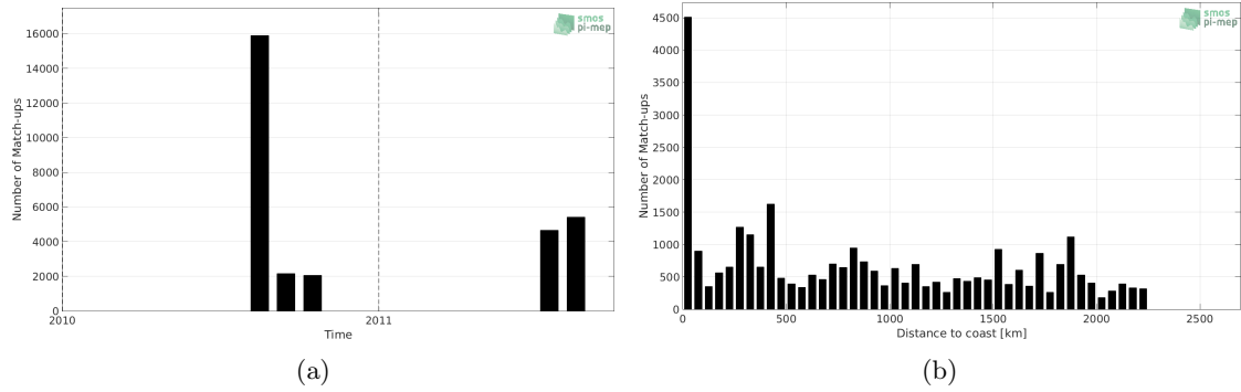
Figure 1: Number of match-ups between TSG-GOSUD-Sailing-ship and SMOS-L3-ICDC-V3-MONTHLY-0.5DEG SSS as a function of time (a) and as function of the distance to coast (b) over the Tropical Pacific Ocean Pi-MEP region and for the full satellite product period.
