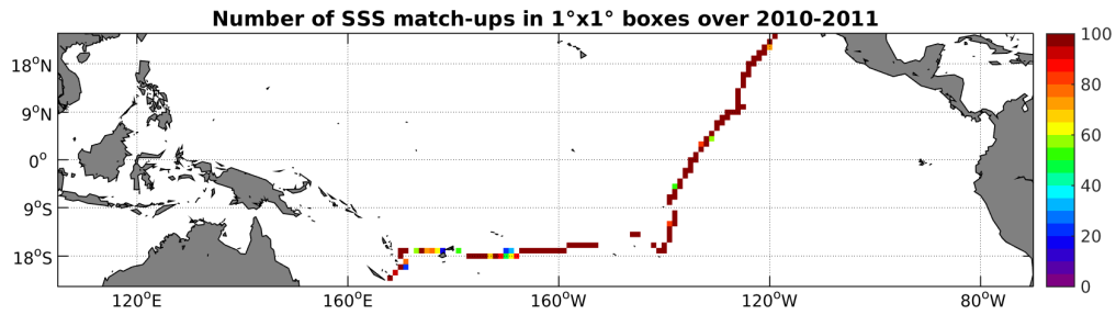
Figure 4: Number of SSS match-ups between TSG-GOSUD-Sailing-ship SSS and the SMOS-L3-ICDC-V3-MONTHLY-0.5DEG SSS product for the Tropical Pacific Ocean Pi-MEP region over 1^\circ \times 1^\circ boxes and for the full satellite product period.
