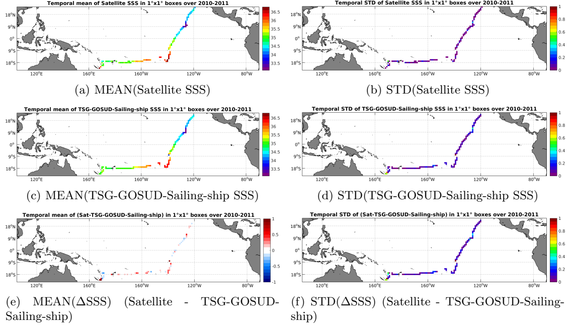
Figure 6: Temporal mean (left) and STD (right) of SSS from SMOS-L3-ICDC-V3-MONTHLY-0.5DEG (top), TSG-GOSUD-Sailing-ship (middle), and of \Delta SSS (Satellite - TSG-GOSUD-Sailing-ship). Only match-up pairs are used to generate these maps.
