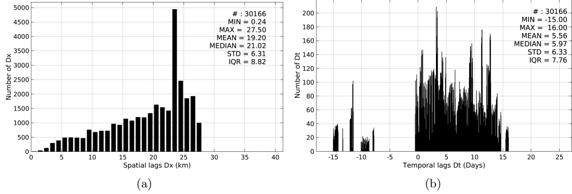
Figure 5: Histograms of the spatial (a) and temporal (b) lags between the time of the TSG-GOSUD-Sailing-ship measurements and the date of the corresponding SMOS-L3-ICDC-V3-MONTHLY-0.5DEG SSS product.
