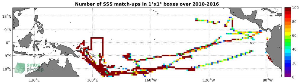
Figure 4: Number of SSS match-ups between TSG (GOSUD-Research-vessel) SSS and the SMOS SSS L3 v3 Monthly (ICDC) SSS product for the Tropical Pacific Ocean Pi-MEP region over 1^\circ \times 1^\circ boxes and for the full satellite product period.
