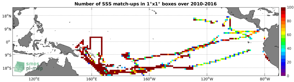
Figure 4: Number of SSS match-ups between TSG (GOSUD-Research-vessel) SSS and the SMOS SSS L3 v3 Monthly (ICDC) SSS product for the Tropical Pacific Ocean Pi-MEP region over 1^\circ \times 1^\circ boxes and for the full satellite product period.
