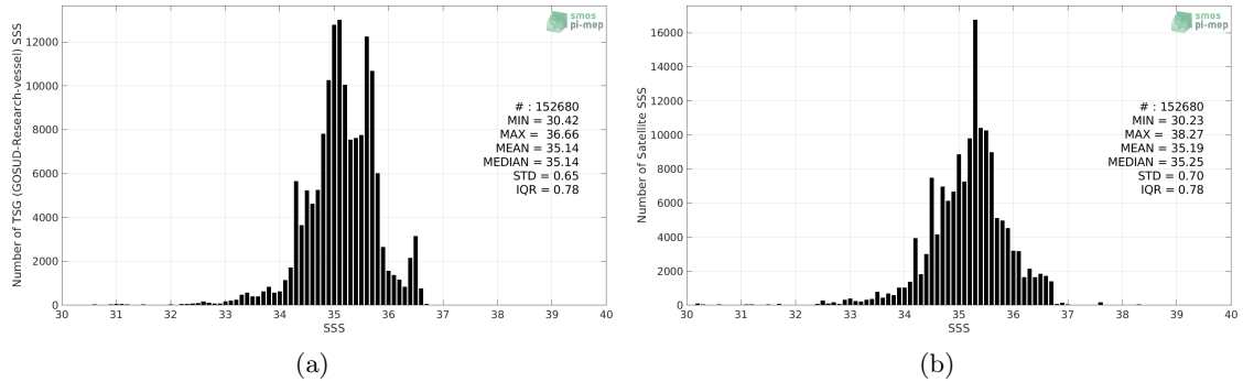
Figure 2: Histograms of SSS from TSG (GOSUD-Research-vessel) (a) and SMOS SSS L3 v3 Monthly (ICDC) (b) considering all match-up pairs per bins of 0.1 over the Tropical Pacific Ocean Pi-MEP region and for the full satellite product period.
