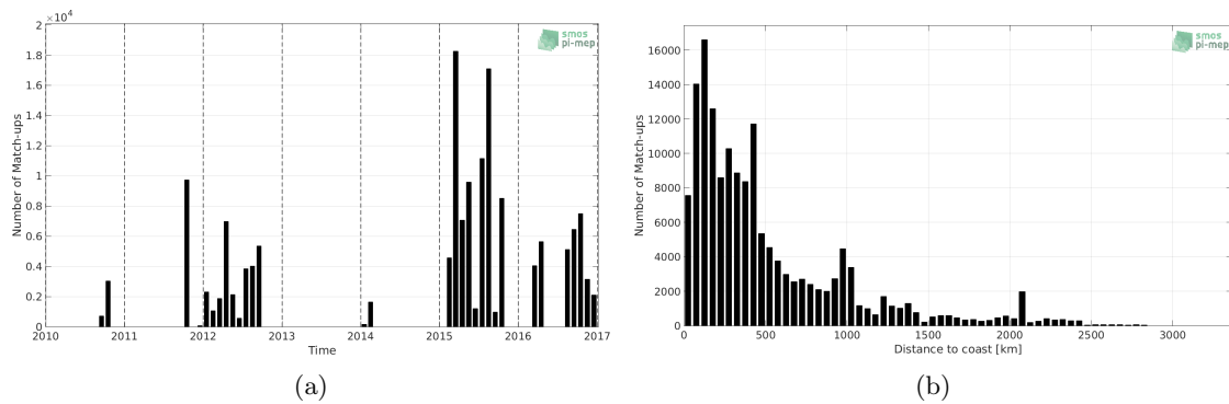
Figure 1: Number of match-ups between TSG-GOSUD-Research-vessel and SMOS-L3-ICDC-V3-MONTHLY-0.5DEG SSS as a function of time (a) and as function of the distance to coast (b) over the Tropical Pacific Ocean Pi-MEP region and for the full satellite product period.
