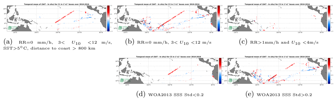
Figure 12: Temporal mean gridded over spatial boxes of size 1^\circ \times 1^\circ of \Delta SSS (SMOS-L3-ICDC-V3-MONTHLY-0.5DEG - TSG-GOSUD-Research-vessel) for 5 different subdatasets corresponding to: RR=0 mm/h, 3 < U_{10} < 12 m/s, SST > 5^\circ\text{C} , distance to coast > 800 km (a), RR=0 mm/h, 3 < U_{10} < 12 m/s (b), RR > 1 mm/h and U_{10} < 4 m/s (c), WOA2013 SSS Std < 0.2 (d), WOA2013 SSS Std > 0.2 (e).
