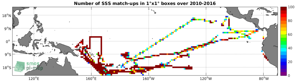
Figure 4: Number of SSS match-ups between TSG-GOSUD-Research-vessel SSS and the SMOS-L3-ICDC-V3-MONTHLY-0.5DEG SSS product for the Tropical Pacific Ocean Pi-MEP region over 1°x1° boxes and for the full satellite product period.
