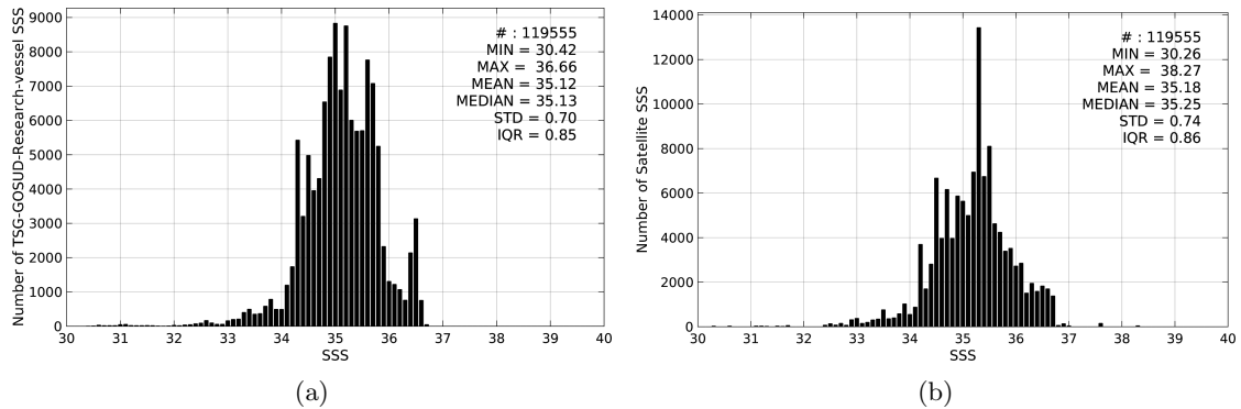
Figure 2: Histograms of SSS from TSG-GOSUD-Research-vessel (a) and SMOS-L3-ICDC-V3-MONTHLY-0.5DEG (b) considering all match-up pairs per bins of 0.1 over the Tropical Pacific Ocean Pi-MEP region and for the full satellite product period.
