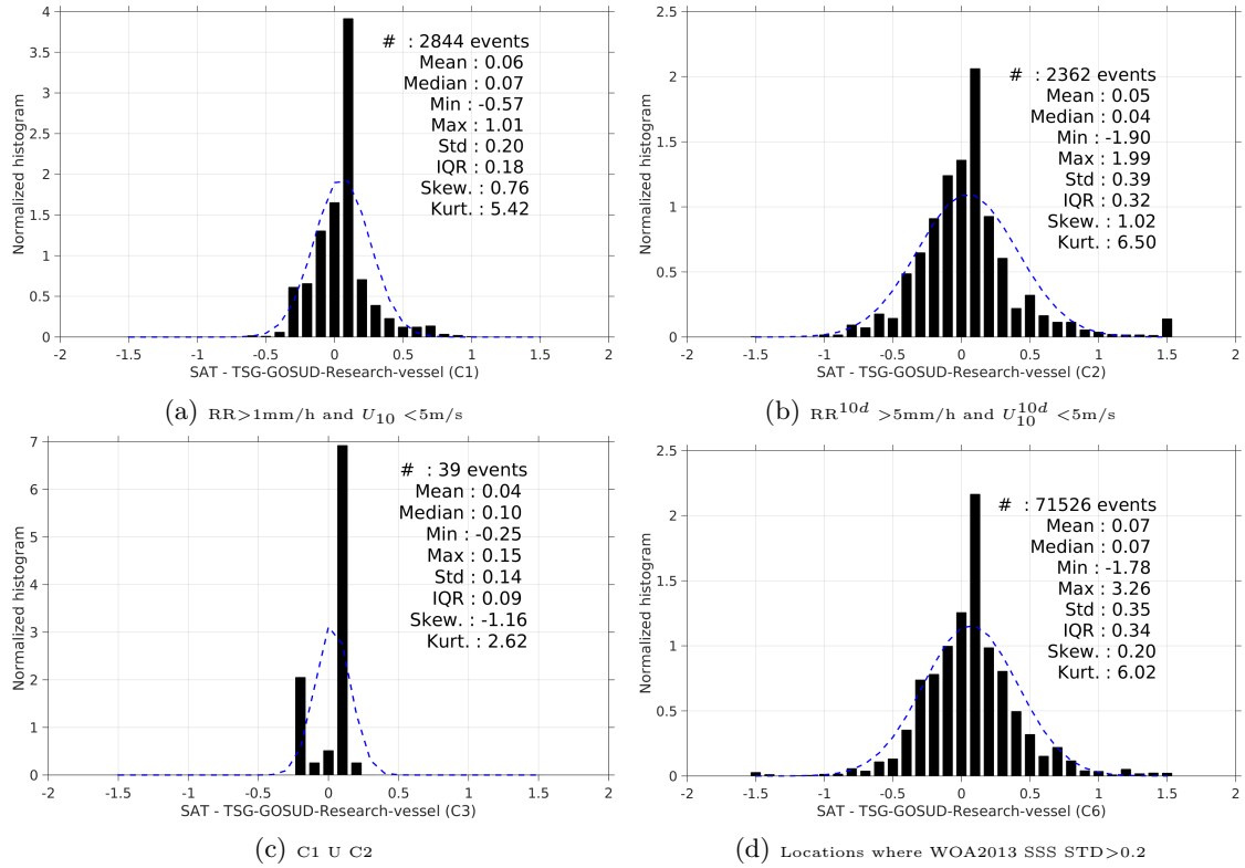
Figure 13: Normalized histogram of \Delta\text{SSS} (SMOS-L3-ICDC-V3-MONTHLY-0.5DEG - TSG-GOSUD-Research-vessel) for 6 different subdatasets corresponding to: RR > 1mm/h and U_{10} < 5\text{m/s} (a), RR^{10d} > 5\text{mm/h} and U_{10}^{10d} < 5\text{m/s} (b), C1 U C2 (c), Locations where WOA2013 SSS STD > 0.2 (d).
