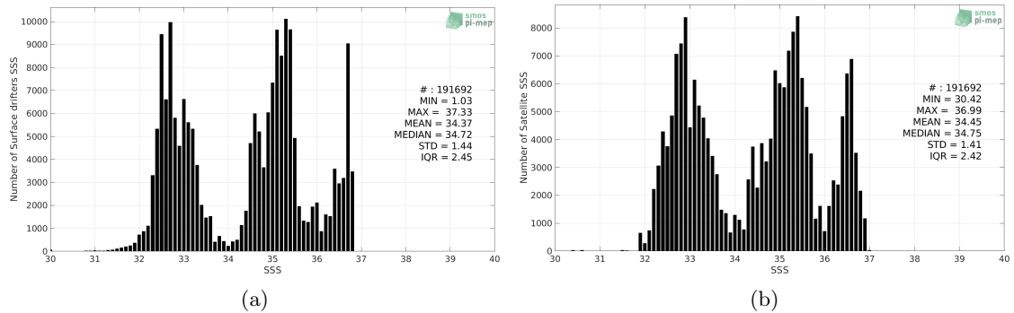
Figure 2: Histograms of SSS from Surface drifters (a) and SMOS SSS L3 v3 Monthly (ICDC) (b) considering all match-up pairs per bins of 0.1 over the Tropical Pacific Ocean Pi-MEP region and for the full satellite product period.
