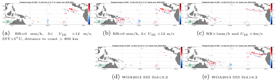
Figure 11: Temporal mean gridded over spatial boxes of size 1^\circ \times 1^\circ of \Delta SSS (SMOS SSS L3 v3 Monthly (ICDC) - Surface drifters) for 5 different subdatasets corresponding to:RR=0 mm/h, 3 < U_{10} < 12 m/s, SST > 5^\circ C , distance to coast > 800 km (a), RR=0 mm/h, 3 < U_{10} < 12 m/s (b), RR>1mm/h and U_{10} < 4 m/s (c), WOA2013 SSS Std<0.2 (d), WOA2013 SSS Std>0.2 (e).
