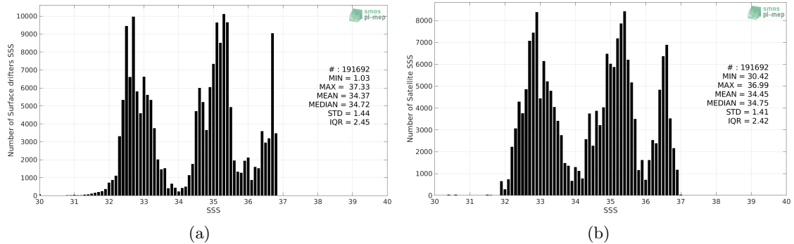
Figure 2: Histograms of SSS from Surface drifters (a) and SMOS SSS L3 v3 Monthly (ICDC) (b) considering all match-up pairs per bins of 0.1 over the Tropical Pacific Ocean Pi-MEP region and for the full satellite product period.
