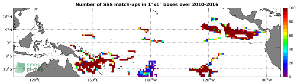
Figure 3: Number of SSS match-ups between Surface drifters SSS and the SMOS SSS L3 v3 Monthly (ICDC) SSS product for the Tropical Pacific Ocean Pi-MEP region over 1^\circ \times 1^\circ boxes and for the full satellite product period.
