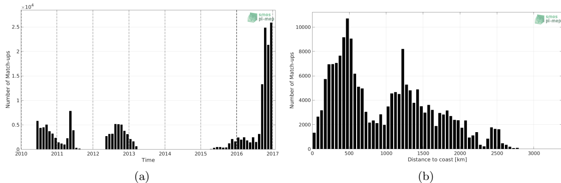
Figure 1: Number of match-ups between Surface drifters and SMOS SSS L3 v3 Monthly (ICDC) SSS as a function of time (a) and as function of the distance to coast (b) over the Tropical Pacific Ocean Pi-MEP region and for the full satellite product period.
