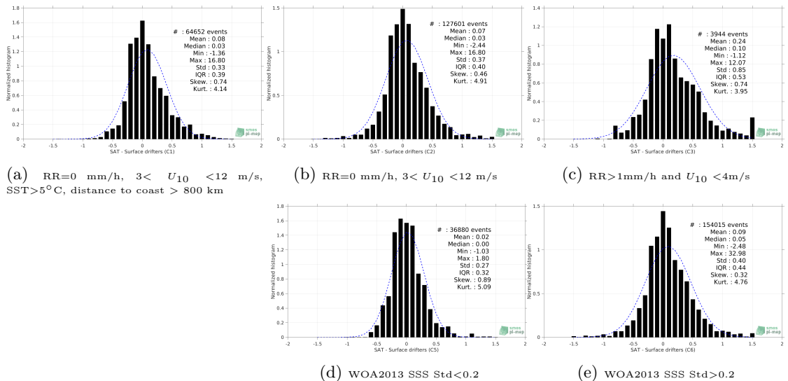
Figure 12: Normalized histogram of ΔSSS (SMOS SSS L3 v3 Monthly (ICDC) - Surface drifters) for 5 different subdatasets corresponding to: RR=0 mm/h, 3 < U_{10} < 12 m/s, SST>5°C, distance to coast > 800 km (a), RR=0 mm/h, 3 < U_{10} < 12 m/s (b), RR>1mm/h and U_{10} < 4m/s (c), WOA2013 SSS Std<0.2 (d), WOA2013 SSS Std>0.2 (e).
