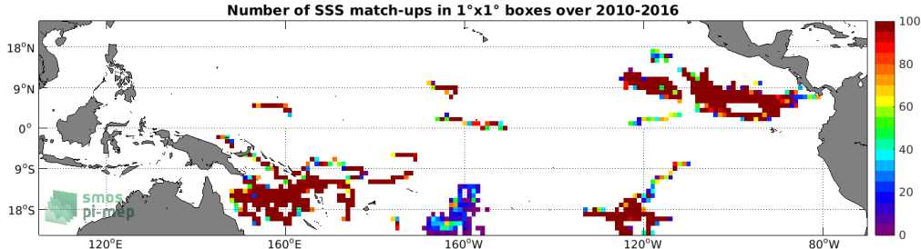
Figure 3: Number of SSS match-ups between Surface drifters SSS and the SMOS SSS L3 v3 Monthly (ICDC) SSS product for the Tropical Pacific Ocean Pi-MEP region over 1^\circ \times 1^\circ boxes and for the full satellite product period.
