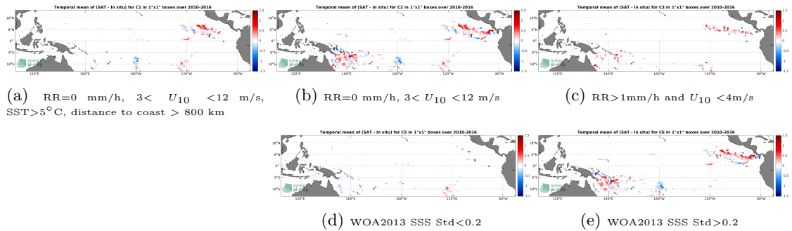
Figure 11: Temporal mean gridded over spatial boxes of size 1°x1° of ΔSSS (SMOS SSS L3 v3 Monthly (ICDC) - Surface drifters) for 5 different subdatasets corresponding to:RR=0 mm/h, 3 < U_{10} < 12 m/s, SST>5°C, distance to coast > 800 km (a), RR=0 mm/h, 3 < U_{10} < 12 m/s (b), RR>1mm/h and U_{10} < 4m/s (c), WOA2013 SSS Std<0.2 (d), WOA2013 SSS Std>0.2 (e).
