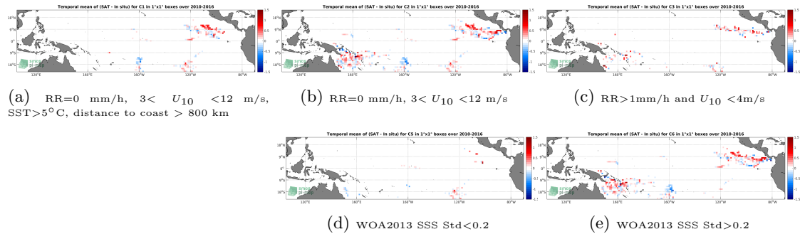
Figure 11: Temporal mean gridded over spatial boxes of size 1^\circ \times 1^\circ of \Delta SSS (SMOS-L3-ICDC-V3-MONTHLY-0.5DEG - Surface drifters) for 5 different subdatasets corresponding to: RR=0 mm/h, 3 < U_{10} < 12 m/s, SST > 5^\circ C , distance to coast > 800 km (a), RR=0 mm/h, 3 < U_{10} < 12 m/s (b), RR > 1 mm/h and U_{10} < 4 m/s (c), WOA2013 SSS Std < 0.2 (d), WOA2013 SSS Std > 0.2 (e).
