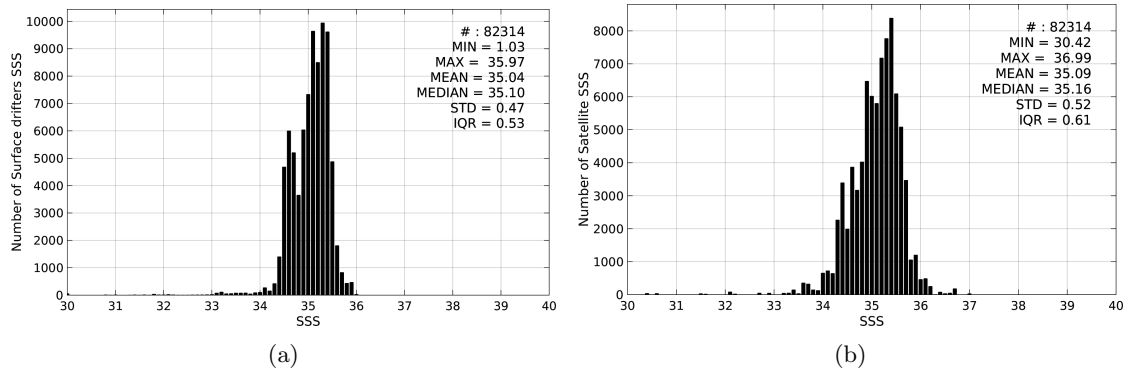
Figure 2: Histograms of SSS from Surface drifters (a) and SMOS-L3-ICDC-V3-MONTHLY-0.5DEG (b) considering all match-up pairs per bins of 0.1 over the Tropical Pacific Ocean Pi-MEP region and for the full satellite product period.
