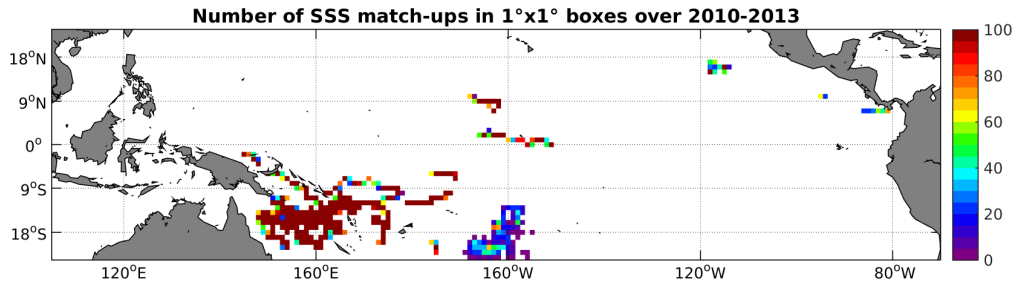
Figure 3: Number of SSS match-ups between Surface drifters SSS and the SMOS-L3-ICDC-V3-MONTHLY-0.5DEG SSS product for the Tropical Pacific Ocean Pi-MEP region over 1^\circ \times 1^\circ boxes and for the full satellite product period.
