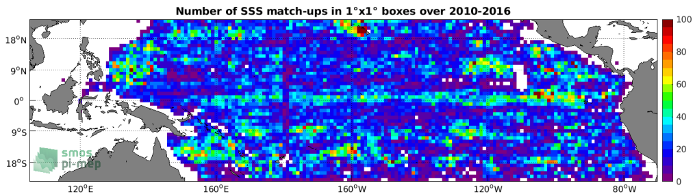
Figure 4: Number of SSS match-ups between Argo SSS and the SMOS SSS L3 v3 Monthly (ICDC) SSS product for the Tropical Pacific Ocean Pi-MEP region over 1°x1° boxes and for the full satellite product period.
