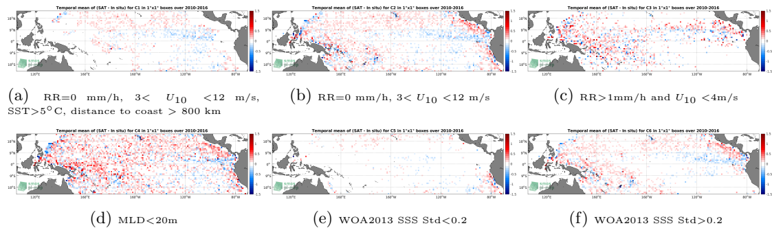
Figure 12: Temporal mean gridded over spatial boxes of size 1^\circ \times 1^\circ of \Delta SSS (SMOS SSS L3 v3 Monthly (ICDC) - Argo) for 6 different subdatasets corresponding to: RR=0 mm/h, 3 < U_{10} < 12 m/s, SST > 5°C, distance to coast > 800 km (a), RR=0 mm/h, 3 < U_{10} < 12 m/s (b), RR > 1mm/h and U_{10} < 4 m/s (c), MLD < 20m (d), WOA2013 SSS Std < 0.2 (e), WOA2013 SSS Std > 0.2 (f).
