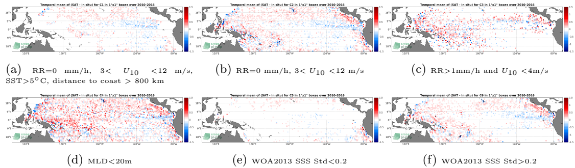
Figure 12: Temporal mean gridded over spatial boxes of size 1^\circ \times 1^\circ of \Delta SSS (SMOS SSS L3 v3 Monthly (ICDC) - Argo) for 6 different subdatasets corresponding to:RR=0 mm/h, 3 < U_{10} < 12 m/s, SST >5^\circ C, distance to coast > 800 km (a), RR=0 mm/h, 3 < U_{10} < 12 m/s (b), RR >1 mm/h and U_{10} < 4 m/s (c),MLD <20 m (d),WOA2013 SSS Std <0.2 (e),WOA2013 SSS Std >0.2 (f).
