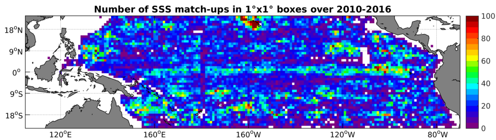
Figure 4: Number of SSS match-ups between Argo SSS and the SMOS-L3-ICDC-V3-MONTHLY-0.5DEG SSS product for the Tropical Pacific Ocean Pi-MEP region over 1^\circ \times 1^\circ boxes and for the full satellite product period.
