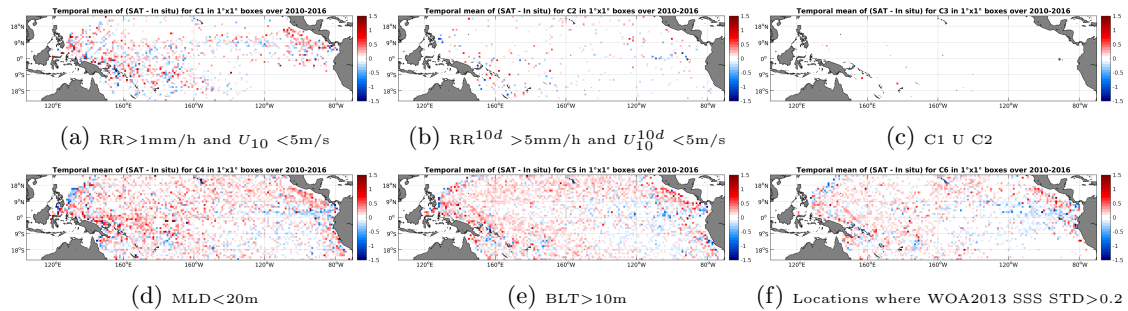
Figure 12: Temporal mean gridded over spatial boxes of size 1^\circ \times 1^\circ of \Delta SSS (SMOS-L3-ICDC-V3-MONTHLY-0.5DEG - Argo) for 6 different subdatasets corresponding to: RR>1mm/h and U_{10} < 5\text{m/s} (a), RR^{10d} > 5\text{mm/h} and U_{10}^{10d} < 5\text{m/s} (b), C1 U C2 (c), MLD<20m (d), BLT>10m (e), Locations where WOA2013 SSS STD>0.2 (f).
