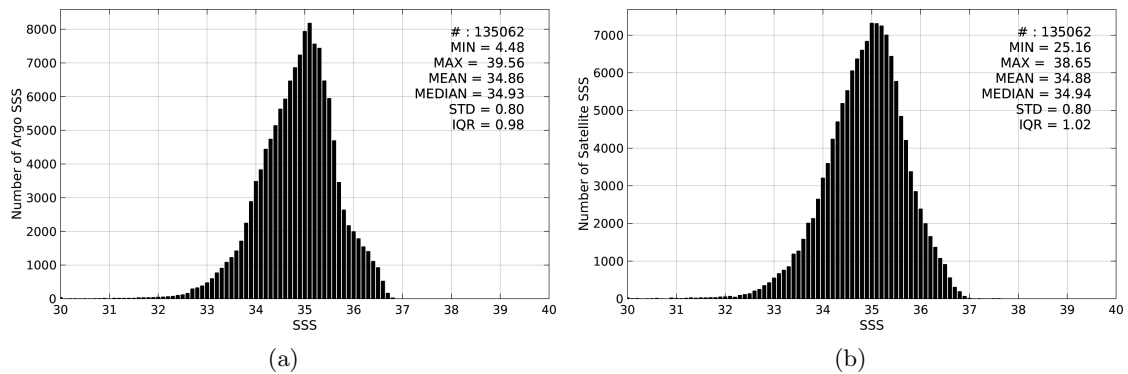
Figure 2: Histograms of SSS from Argo (a) and SMOS-L3-ICDC-V3-MONTHLY-0.5DEG (b) considering all match-up pairs per bins of 0.1 over the Tropical Pacific Ocean Pi-MEP region and for the full satellite product period.
