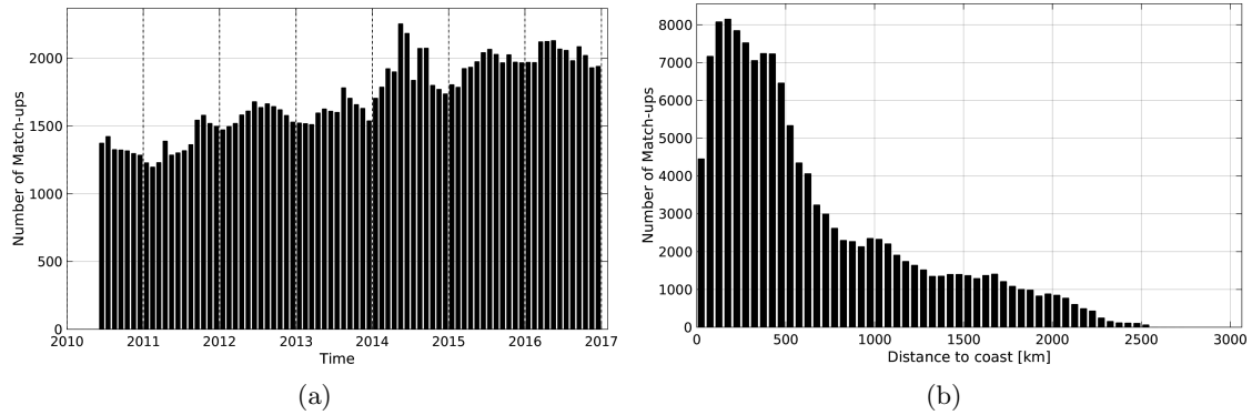
Figure 1: Number of match-ups between Argo and SMOS-L3-ICDC-V3-MONTHLY-0.5DEG SSS as a function of time (a) and as function of the distance to coast (b) over the Tropical Pacific Ocean Pi-MEP region and for the full satellite product period.
