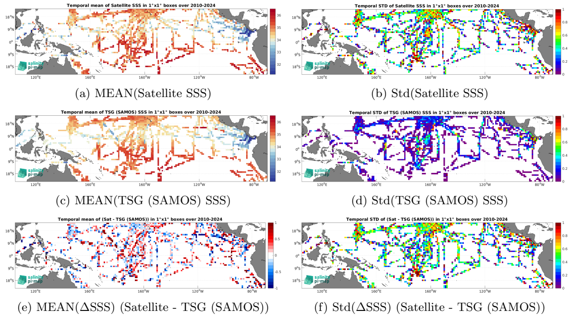
Figure 7: Temporal mean (left) and Std (right) of SSS from SMOS SSS L2Q v331 - With FLAG (CMEMS-CATDS-CPDC) (top), TSG (SAMOS) (middle), and of \Delta SSS (Satellite - TSG (SAMOS)). Only match-up pairs are used to generate these maps.
