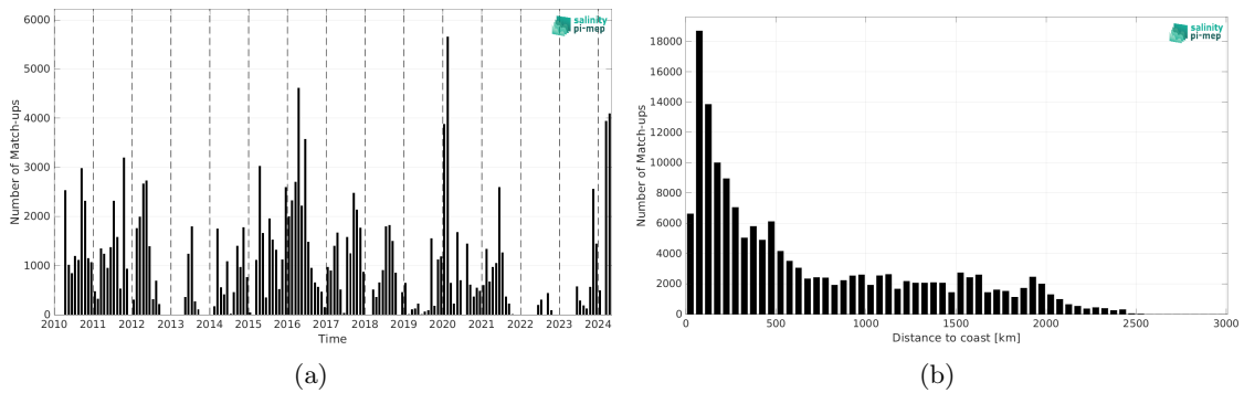
Figure 2: Number of match-ups between TSG (SAMOS) and SMOS SSS L2Q v331 - With FLAG (CMEMS-CATDS-CPDC) SSS as a function of time (a) and as function of the distance to coast (b) over the Tropical Pacific Ocean Pi-MEP region and for the full satellite product period.
