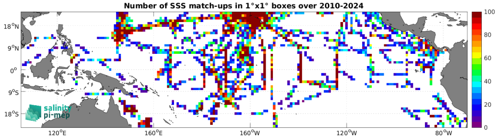
Figure 5: Number of SSS match-ups between TSG (SAMOS) SSS and the SMOS SSS L2Q v331 - With FLAG (CMEMS-CATDS-CPDC) SSS product for the Tropical Pacific Ocean Pi-MEP region over 1^\circ \times 1^\circ boxes and for the full satellite product period.
