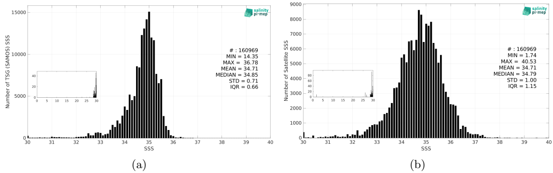
Figure 3: Histograms of SSS from TSG (SAMOS) (a) and SMOS SSS L2Q v331 - With FLAG (CMEMS-CATDS-CPDC) (b) considering all match-up pairs per bins of 0.1 over the Tropical Pacific Ocean Pi-MEP region and for the full satellite product period.
