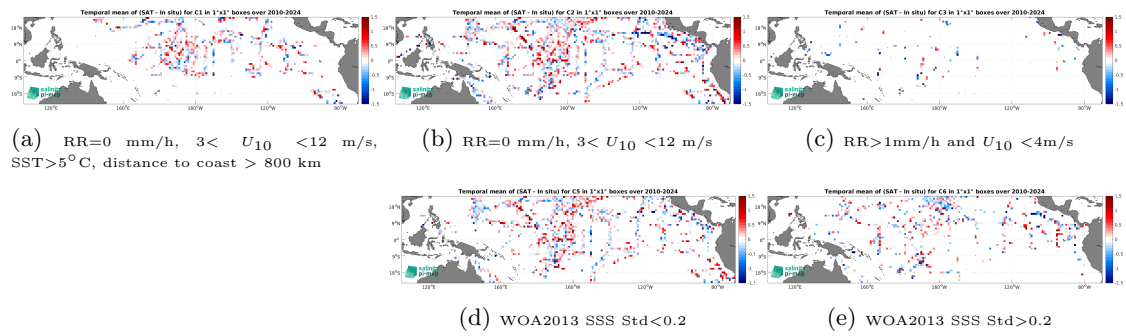
Figure 14: Temporal mean gridded over spatial boxes of size 1^\circ \times 1^\circ of \Delta SSS (SMOS SSS L2Q v331 - With FLAG (CMEMS-CATDS-CPDC) - TSG (SAMOS)) for 5 different subdatasets corresponding to: RR=0 mm/h, 3 < U_{10} < 12 m/s, SST > 5°C, distance to coast > 800 km (a), RR=0 mm/h, 3 < U_{10} < 12 m/s (b), RR > 1mm/h and U_{10} < 4 m/s (c), WOA2013 SSS Std < 0.2 (d), WOA2013 SSS Std > 0.2 (e).
