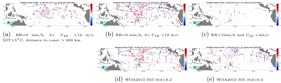
Figure 12: Temporal mean gridded over spatial boxes of size 1^{\circ}\times 1^{\circ} of \Delta\text{SSS} (SMOS SSS L2Q v331 - With FLAG (CMEMS-CATDS-CPDC) - TSG (SAMOS)) for 5 different subdatasets corresponding to: RR=0 mm/h, 3 < U_{10} < 12 m/s, SST > 5^{\circ}\text{C} , distance to coast > 800 km (a), RR=0 mm/h, 3 < U_{10} < 12 m/s (b), RR > 1 mm/h and U_{10} < 4 m/s (c), WOA2013 SSS Std < 0.2 (d), WOA2013 SSS Std > 0.2 (e).
