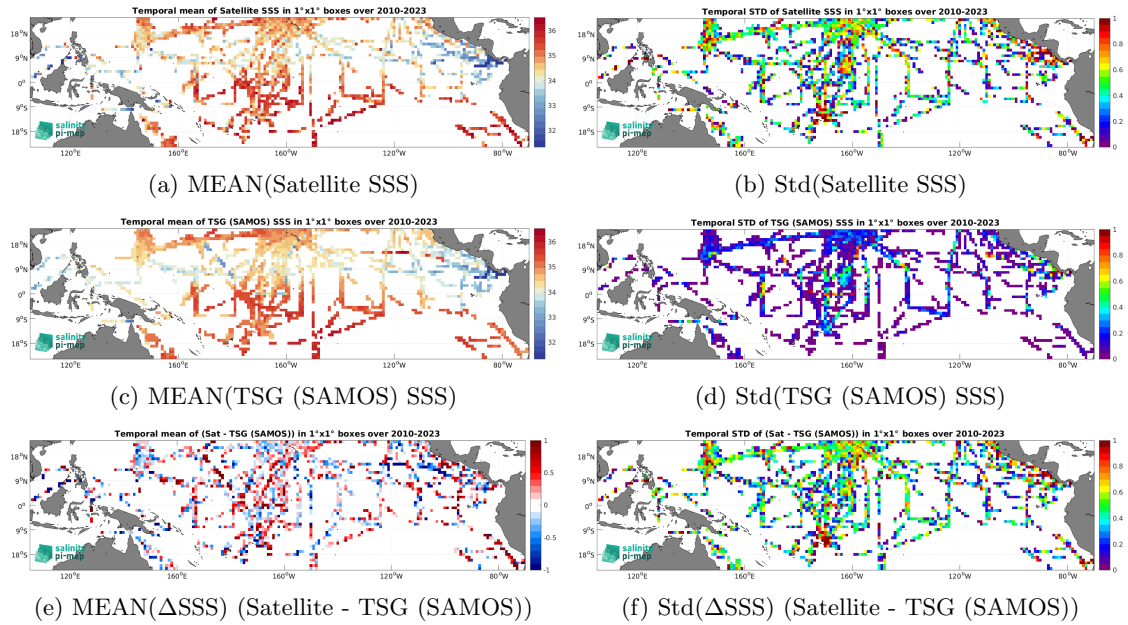
Figure 6: Temporal mean (left) and Std (right) of SSS from SMOS SSS L2Q v331 - With FLAG (CMEMS-CATDS-CPDC) (top), TSG (SAMOS) (middle), and of \Delta SSS (Satellite - TSG (SAMOS)). Only match-up pairs are used to generate these maps.
