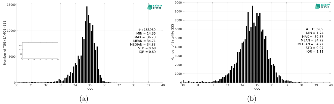
Figure 2: Histograms of SSS from TSG (SAMOS) (a) and SMOS SSS L2Q v331 - With FLAG (CMEMS-CATDS-CPDC) (b) considering all match-up pairs per bins of 0.1 over the Tropical Pacific Ocean Pi-MEP region and for the full satellite product period.
