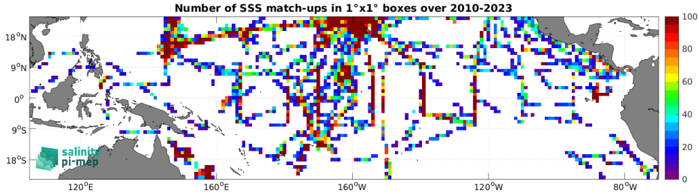
Figure 4: Number of SSS match-ups between TSG (SAMOS) SSS and the SMOS SSS L2Q v331 - With FLAG (CMEMS-CATDS-CPDC) SSS product for the Tropical Pacific Ocean Pi-MEP region over 1^\circ \times 1^\circ boxes and for the full satellite product period.
