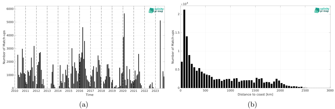
Figure 1: Number of match-ups between TSG (SAMOS) and SMOS SSS L2Q v331 - With FLAG (CMEMS-CATDS-CPDC) SSS as a function of time (a) and as function of the distance to coast (b) over the Tropical Pacific Ocean Pi-MEP region and for the full satellite product period.
