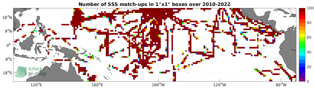
Figure 4: Number of SSS match-ups between TSG (SAMOS) SSS and the SMOS SSS L2Q v331 - With FLAG (CMEMS-CATDS-CPDC) SSS product for the Tropical Pacific Ocean Pi-MEP region over 1^\circ \times 1^\circ boxes and for the full satellite product period.
