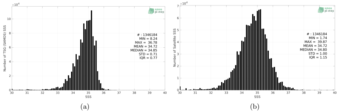
Figure 2: Histograms of SSS from TSG (SAMOS) (a) and SMOS SSS L2Q v331 - With FLAG (CMEMS-CATDS-CPDC) (b) considering all match-up pairs per bins of 0.1 over the Tropical Pacific Ocean Pi-MEP region and for the full satellite product period.
