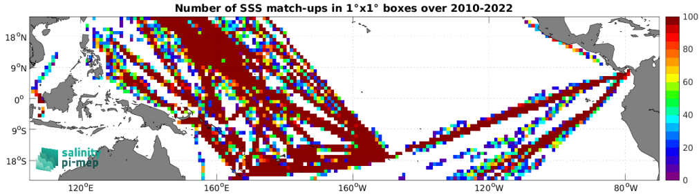
Figure 5: Number of SSS match-ups between TSG (LEGOS-DM) SSS and the SMOS SSS L2Q v331 - With FLAG (CMEMS-CATDS-CPDC) SSS product for the Tropical Pacific Ocean Pi-MEP region over 1^\circ \times 1^\circ boxes and for the full satellite product period.
