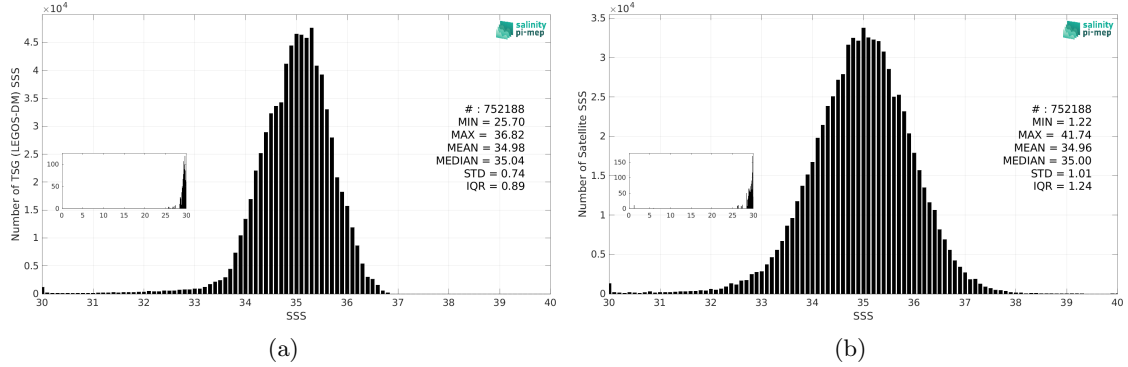
Figure 3: Histograms of SSS from TSG (LEGOS-DM) (a) and SMOS SSS L2Q v331 - With FLAG (CMEMS-CATDS-CPDC) (b) considering all match-up pairs per bins of 0.1 over the Tropical Pacific Ocean Pi-MEP region and for the full satellite product period.
