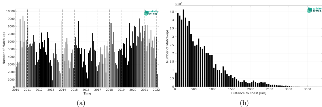
Figure 2: Number of match-ups between TSG (LEGOS-DM) and SMOS SSS L2Q v331 - With FLAG (CMEMS-CATDS-CPDC) SSS as a function of time (a) and as function of the distance to coast (b) over the Tropical Pacific Ocean Pi-MEP region and for the full satellite product period.
