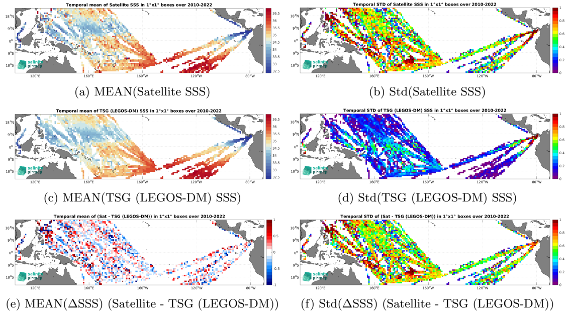
Figure 7: Temporal mean (left) and Std (right) of SSS from SMOS SSS L2Q v331 - With FLAG (CMEMS-CATDS-CPDC) (top), TSG (LEGOS-DM) (middle), and of \Delta SSS (Satellite - TSG (LEGOS-DM)). Only match-up pairs are used to generate these maps.
