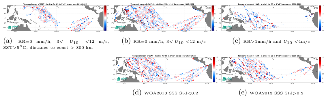
Figure 14: Temporal mean gridded over spatial boxes of size 1^\circ \times 1^\circ of \Delta SSS (SMOS SSS L2Q v331 - With FLAG (CMEMS-CATDS-CPDC) - TSG (LEGOS-DM)) for 5 different subdatasets corresponding to: RR=0 mm/h, 3 < U_{10} < 12 m/s, SST > 5^\circ\text{C} , distance to coast > 800 km (a), RR=0 mm/h, 3 < U_{10} < 12 m/s (b), RR > 1 mm/h and U_{10} < 4 m/s (c), WOA2013 SSS Std < 0.2 (d), WOA2013 SSS Std > 0.2 (e).
