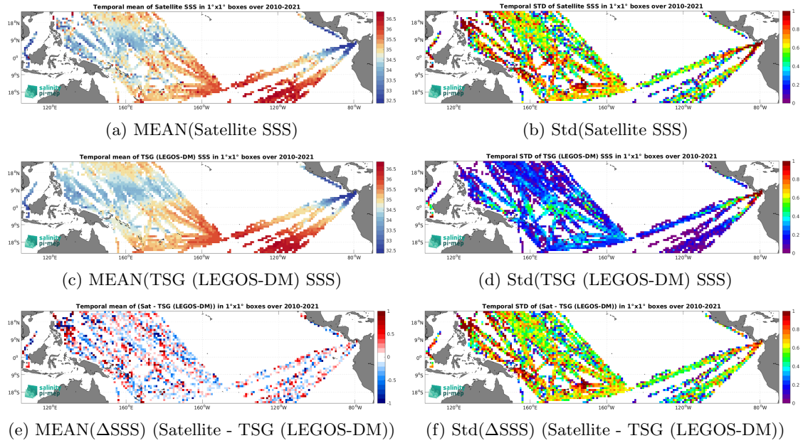
Figure 6: Temporal mean (left) and Std (right) of SSS from SMOS SSS L2Q v331 - With FLAG (CMEMS-CATDS-CPDC) (top), TSG (LEGOS-DM) (middle), and of \Delta SSS (Satellite - TSG (LEGOS-DM)). Only match-up pairs are used to generate these maps.
