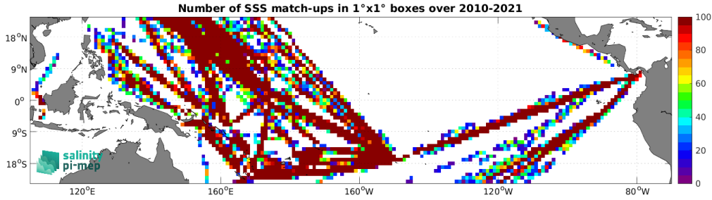
Figure 4: Number of SSS match-ups between TSG (LEGOS-DM) SSS and the SMOS SSS L2Q v331 - With FLAG (CMEMS-CATDS-CPDC) SSS product for the Tropical Pacific Ocean Pi-MEP region over 1^\circ \times 1^\circ boxes and for the full satellite product period.
