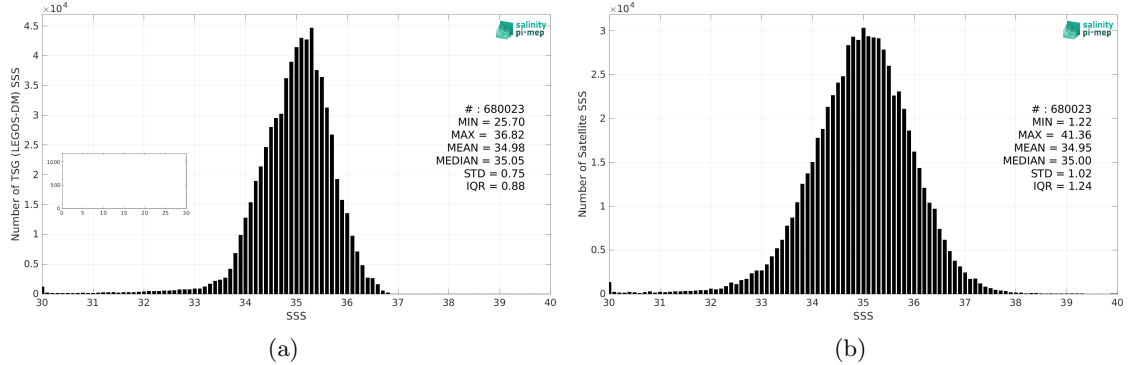
Figure 2: Histograms of SSS from TSG (LEGOS-DM) (a) and SMOS SSS L2Q v331 - With FLAG (CMEMS-CATDS-CPDC) (b) considering all match-up pairs per bins of 0.1 over the Tropical Pacific Ocean Pi-MEP region and for the full satellite product period.
