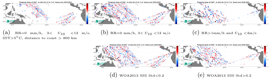
Figure 12: Temporal mean gridded over spatial boxes of size 1^\circ \times 1^\circ of \Delta\text{SSS} (SMOS SSS L2Q v331 - With FLAG (CMEMS-CATDS-CPDC) - TSG (LEGOS-DM)) for 5 different subdatasets corresponding to: RR=0 mm/h, 3 < U_{10} < 12 m/s, SST > 5^\circ\text{C} , distance to coast > 800 km (a), RR=0 mm/h, 3 < U_{10} < 12 m/s (b), RR > 1 mm/h and U_{10} < 4 m/s (c), WOA2013 SSS Std < 0.2 (d), WOA2013 SSS Std > 0.2 (e).
