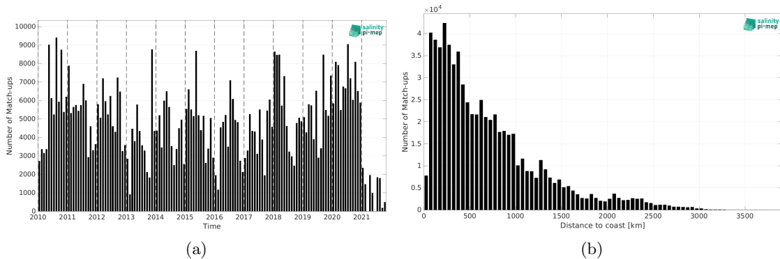
Figure 1: Number of match-ups between TSG (LEGOS-DM) and SMOS SSS L2Q v331 - With FLAG (CMEMS-CATDS-CPDC) SSS as a function of time (a) and as function of the distance to coast (b) over the Tropical Pacific Ocean Pi-MEP region and for the full satellite product period.
