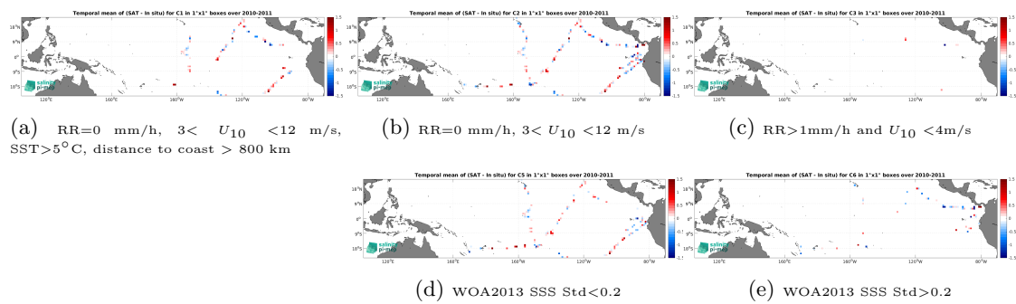
Figure 14: Temporal mean gridded over spatial boxes of size 1^\circ \times 1^\circ of \Delta SSS (SMOS SSS L2Q v331 - With FLAG (CMEMS-CATDS-CPDC) - TSG (GOSUD-Sailing-ship)) for 5 different subdatasets corresponding to:RR=0 mm/h, 3 < U_{10} < 12 m/s, SST > 5^\circ\text{C} , distance to coast > 800 km (a), RR=0 mm/h, 3 < U_{10} < 12 m/s (b), RR > 1 mm/h and U_{10} < 4 m/s (c), WOA2013 SSS Std < 0.2 (d), WOA2013 SSS Std > 0.2 (e).
