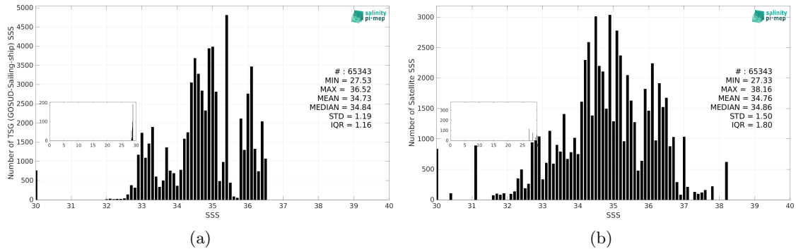
Figure 3: Histograms of SSS from TSG (GOSUD-Sailing-ship) (a) and SMOS SSS L2Q v331 - With FLAG (CMEMS-CATDS-CPDC) (b) considering all match-up pairs per bins of 0.1 over the Tropical Pacific Ocean Pi-MEP region and for the full satellite product period.
