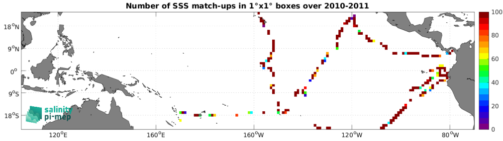
Figure 4: Number of SSS match-ups between TSG (GOSUD-Sailing-ship) SSS and the SMOS SSS L2Q v331 - With FLAG (CMEMS-CATDS-CPDC) SSS product for the Tropical Pacific Ocean Pi-MEP region over 1^\circ \times 1^\circ boxes and for the full satellite product period.
