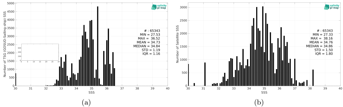
Figure 2: Histograms of SSS from TSG (GOSUD-Sailing-ship) (a) and SMOS SSS L2Q v331 - With FLAG (CMEMS-CATDS-CPDC) (b) considering all match-up pairs per bins of 0.1 over the Tropical Pacific Ocean Pi-MEP region and for the full satellite product period.
