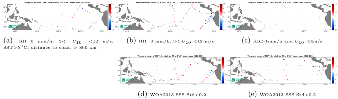
Figure 12: Temporal mean gridded over spatial boxes of size 1^{\circ}\times 1^{\circ} of \Delta SSS (SMOS SSS L2Q v331 - With FLAG (CMEMS-CATDS-CPDC) - TSG (GOSUD-Sailing-ship)) for 5 different subdatasets corresponding to:RR=0 mm/h, 3 < U_{10} < 12 m/s, SST >5^{\circ}\text{C} , distance to coast > 800 km (a), RR=0 mm/h, 3 < U_{10} < 12 m/s (b), RR >1 mm/h and U_{10} < 4 m/s (c), WOA2013 SSS Std <0.2 (d), WOA2013 SSS Std >0.2 (e).
