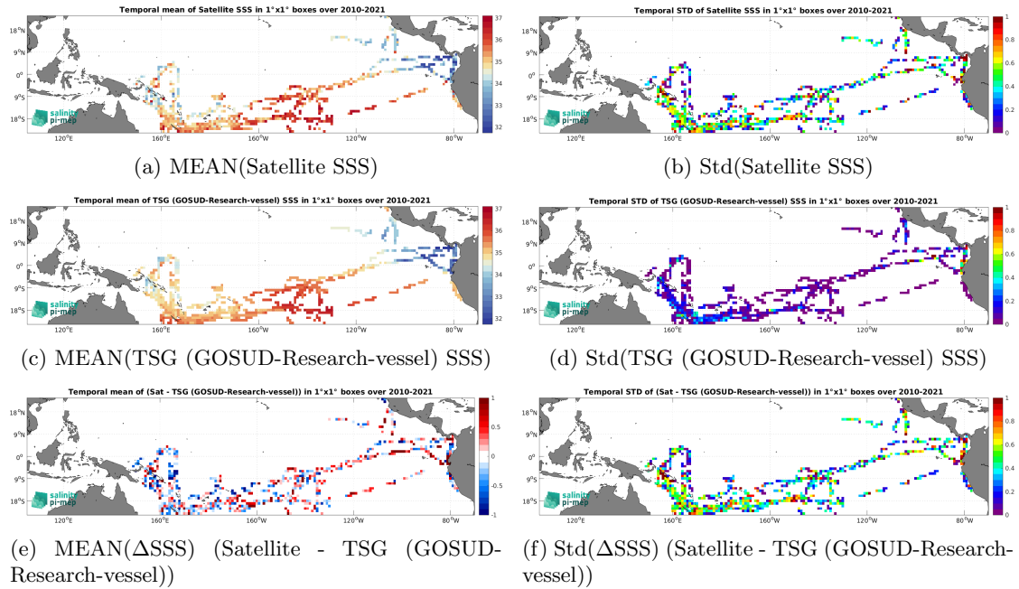
Figure 7: Temporal mean (left) and Std (right) of SSS from SMOS SSS L2Q v331 - With FLAG (CMEMS-CATDS-CPDC) (top), TSG (GOSUD-Research-vessel) (middle), and of \Delta SSS (Satellite - TSG (GOSUD-Research-vessel)). Only match-up pairs are used to generate these maps.
