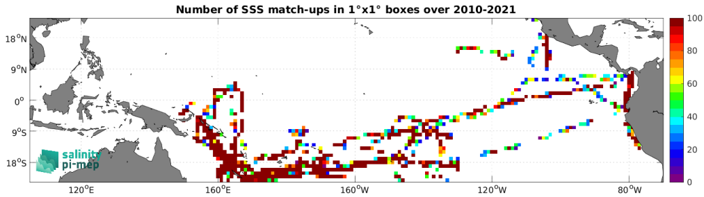
Figure 5: Number of SSS match-ups between TSG (GOSUD-Research-vessel) SSS and the SMOS SSS L2Q v331 - With FLAG (CMEMS-CATDS-CPDC) SSS product for the Tropical Pacific Ocean Pi-MEP region over 1^\circ \times 1^\circ boxes and for the full satellite product period.
