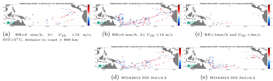
Figure 14: Temporal mean gridded over spatial boxes of size 1^\circ \times 1^\circ of \Delta SSS (SMOS SSS L2Q v331 - With FLAG (CMEMS-CATDS-CPDC) - TSG (GOSUD-Research-vessel)) for 5 different subdatasets corresponding to:RR=0 mm/h, 3 < U_{10} < 12 m/s, SST > 5^\circ\text{C} , distance to coast > 800 km (a), RR=0 mm/h, 3 < U_{10} < 12 m/s (b), RR > 1 mm/h and U_{10} < 4 m/s (c), WOA2013 SSS Std < 0.2 (d), WOA2013 SSS Std > 0.2 (e).
