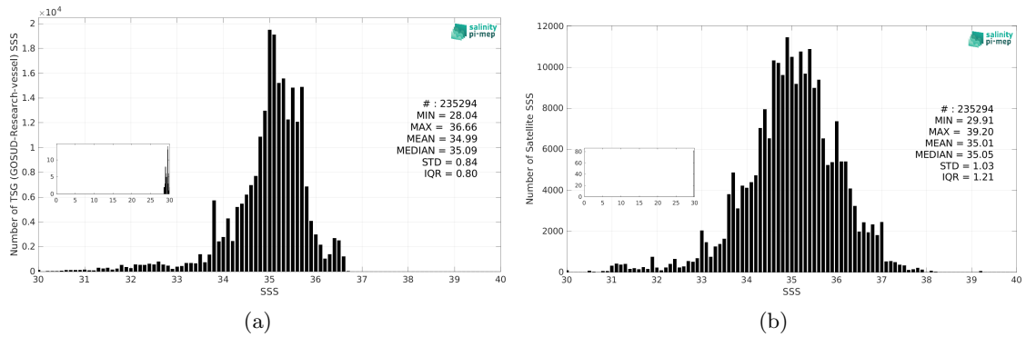
Figure 3: Histograms of SSS from TSG (GOSUD-Research-vessel) (a) and SMOS SSS L2Q v331 - With FLAG (CMEMS-CATDS-CPDC) (b) considering all match-up pairs per bins of 0.1 over the Tropical Pacific Ocean Pi-MEP region and for the full satellite product period.
