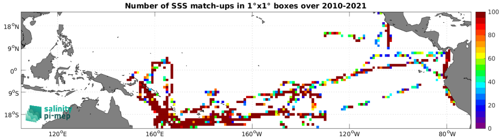
Figure 4: Number of SSS match-ups between TSG (GOSUD-Research-vessel) SSS and the SMOS SSS L2Q v331 - With FLAG (CMEMS-CATDS-CPDC) SSS product for the Tropical Pacific Ocean Pi-MEP region over 1^\circ \times 1^\circ boxes and for the full satellite product period.
