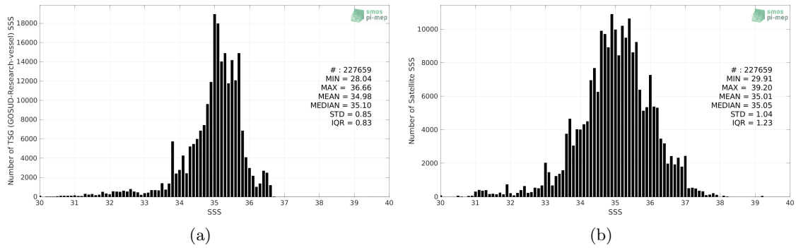
Figure 2: Histograms of SSS from TSG (GOSUD-Research-vessel) (a) and SMOS SSS L2Q v331 - With FLAG (CMEMS-CATDS-CPDC) (b) considering all match-up pairs per bins of 0.1 over the Tropical Pacific Ocean Pi-MEP region and for the full satellite product period.
