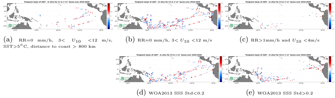
Figure 12: Temporal mean gridded over spatial boxes of size 1^{\circ}\times 1^{\circ} of \Delta SSS (SMOS SSS L2Q v331 - With FLAG (CMEMS-CATDS-CPDC) - TSG (GOSUD-Research-vessel)) for 5 different subdatasets corresponding to:RR=0 mm/h, 3 < U_{10} < 12 m/s, SST >5^{\circ}\text{C} , distance to coast > 800 km (a), RR=0 mm/h, 3 < U_{10} < 12 m/s (b), RR >1 mm/h and U_{10} < 4 m/s (c), WOA2013 SSS Std <0.2 (d), WOA2013 SSS Std >0.2 (e).
