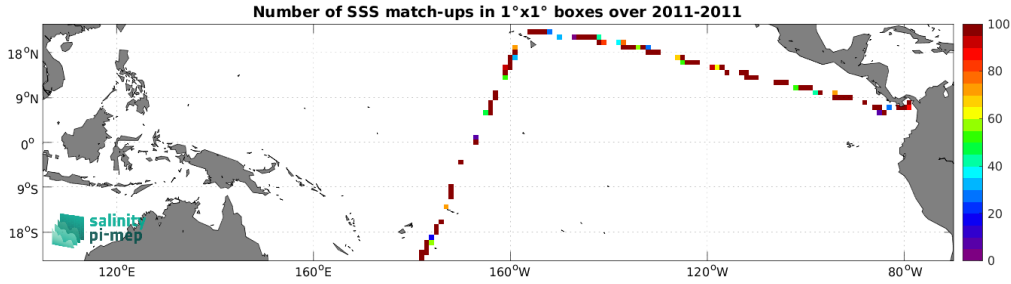
Figure 5: Number of SSS match-ups between TSG (CSIC-UTM) SSS and the SMOS SSS L2Q v331 - With FLAG (CMEMS-CATDS-CPDC) SSS product for the Tropical Pacific Ocean Pi-MEP region over 1^\circ \times 1^\circ boxes and for the full satellite product period.
