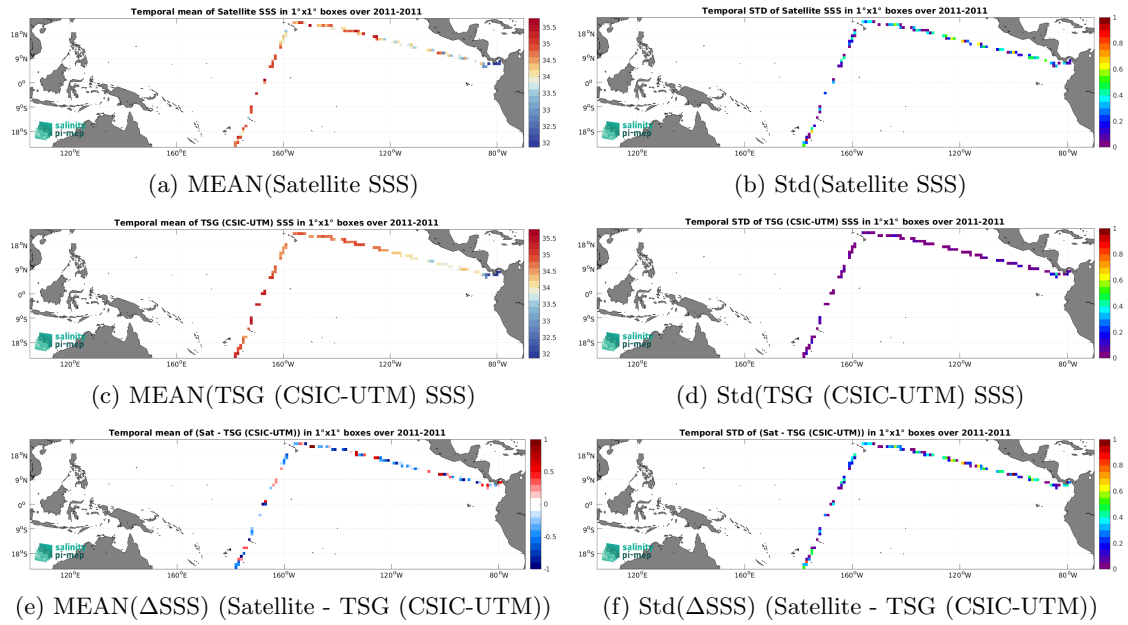
Figure 7: Temporal mean (left) and Std (right) of SSS from SMOS SSS L2Q v331 - With FLAG (CMEMS-CATDS-CPDC) (top), TSG (CSIC-UTM) (middle), and of \Delta SSS (Satellite - TSG (CSIC-UTM)). Only match-up pairs are used to generate these maps.
