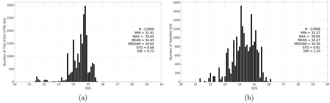
Figure 3: Histograms of SSS from TSG (CSIC-UTM) (a) and SMOS SSS L2Q v331 - With FLAG (CMEMS-CATDS-CPDC) (b) considering all match-up pairs per bins of 0.1 over the Tropical Pacific Ocean Pi-MEP region and for the full satellite product period.
