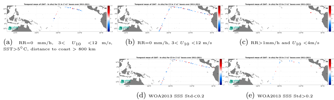
Figure 14: Temporal mean gridded over spatial boxes of size 1^\circ \times 1^\circ of \Delta\text{SSS} (SMOS SSS L2Q v331 - With FLAG (CMEMS-CATDS-CPDC) - TSG (CSIC-UTM)) for 5 different subdatasets corresponding to:RR=0 mm/h, 3 < U_{10} < 12 m/s, SST>5°C, distance to coast > 800 km (a), RR=0 mm/h, 3 < U_{10} < 12 m/s (b), RR>1mm/h and U_{10} < 4 m/s (c), WOA2013 SSS Std<0.2 (d), WOA2013 SSS Std>0.2 (e).
