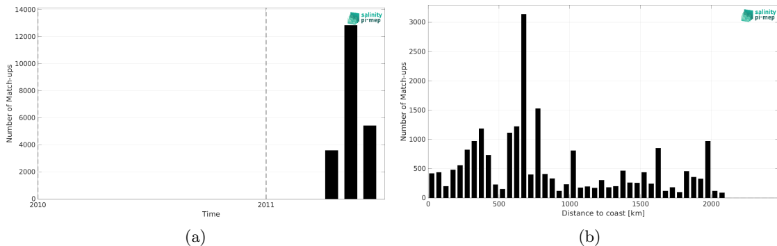
Figure 1: Number of match-ups between TSG (CSIC-UTM) and SMOS SSS L2Q v331 - With FLAG (CMEMS-CATDS-CPDC) SSS as a function of time (a) and as function of the distance to coast (b) over the Tropical Pacific Ocean Pi-MEP region and for the full satellite product period.
