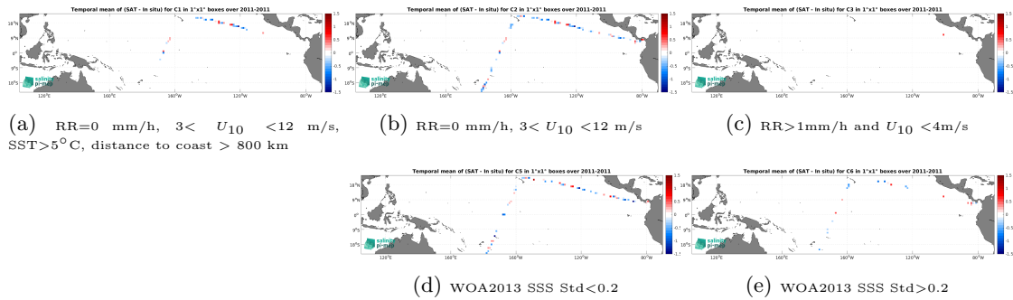
Figure 12: Temporal mean gridded over spatial boxes of size 1^{\circ}\times 1^{\circ} of \Delta\text{SSS} (SMOS SSS L2Q v331 - With FLAG (CMEMS-CATDS-CPDC) - TSG (CSIC-UTM)) for 5 different subdatasets corresponding to:RR=0 mm/h, 3 < U_{10} < 12 m/s, SST >5^{\circ}\text{C} , distance to coast > 800 km (a), RR=0 mm/h, 3 < U_{10} < 12 m/s (b), RR >1 mm/h and U_{10} < 4 m/s (c), WOA2013 SSS Std <0.2 (d), WOA2013 SSS Std >0.2 (e).
