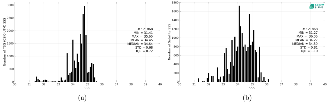
Figure 2: Histograms of SSS from TSG (CSIC-UTM) (a) and SMOS SSS L2Q v331 - With FLAG (CMEMS-CATDS-CPDC) (b) considering all match-up pairs per bins of 0.1 over the Tropical Pacific Ocean Pi-MEP region and for the full satellite product period.
