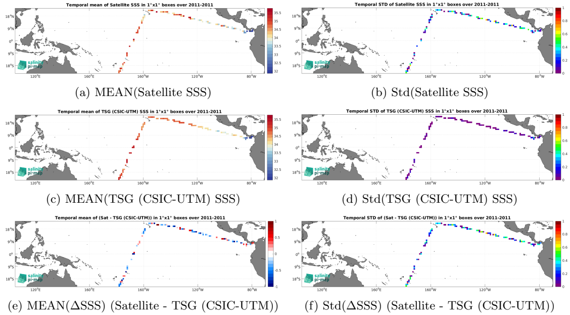
Figure 6: Temporal mean (left) and Std (right) of SSS from SMOS SSS L2Q v331 - With FLAG (CMEMS-CATDS-CPDC) (top), TSG (CSIC-UTM) (middle), and of \Delta SSS (Satellite - TSG (CSIC-UTM)). Only match-up pairs are used to generate these maps.
