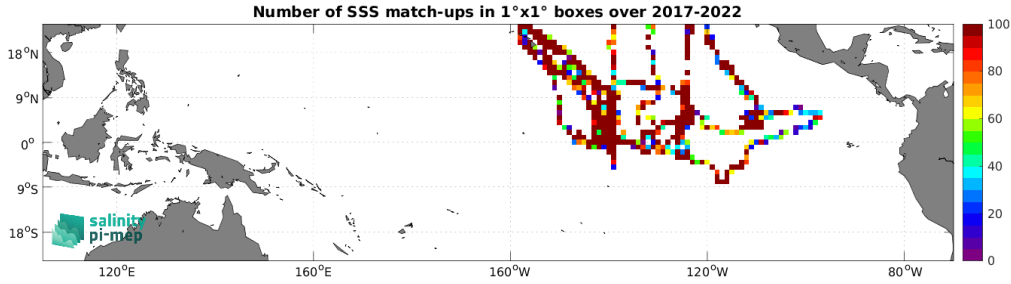
Figure 5: Number of SSS match-ups between Saildrone SSS and the SMOS SSS L2Q v331 - With FLAG (CMEMS-CATDS-CPDC) SSS product for the Tropical Pacific Ocean Pi-MEP region over 1^\circ \times 1^\circ boxes and for the full satellite product period.
