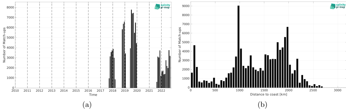
Figure 2: Number of match-ups between Saildrone and SMOS SSS L2Q v331 - With FLAG (CMEMS-CATDS-CPDC) SSS as a function of time (a) and as function of the distance to coast (b) over the Tropical Pacific Ocean Pi-MEP region and for the full satellite product period.
