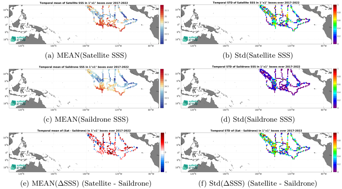
Figure 7: Temporal mean (left) and Std (right) of SSS from SMOS SSS L2Q v331 - With FLAG (CMEMS-CATDS-CPDC) (top), Saildrone (middle), and of \Delta SSS (Satellite - Saildrone). Only match-up pairs are used to generate these maps.
