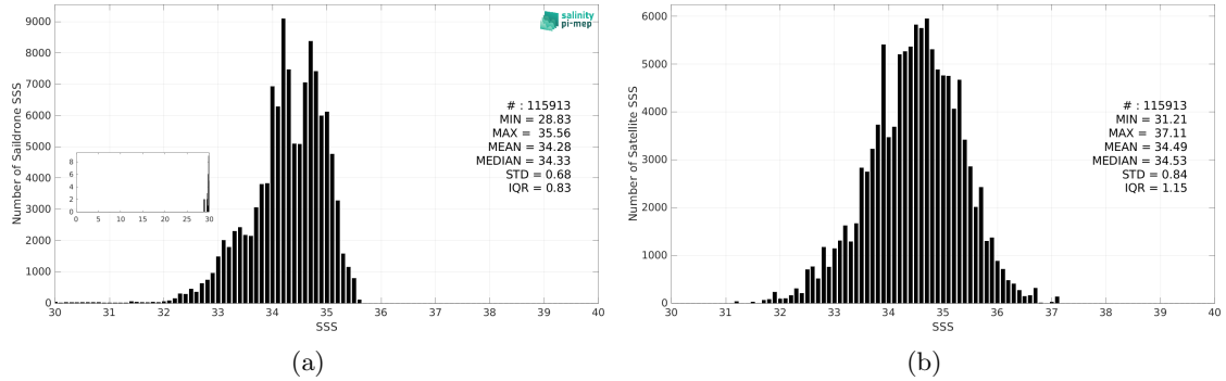
Figure 3: Histograms of SSS from Saildrone (a) and SMOS SSS L2Q v331 - With FLAG (CMEMS-CATDS-CPDC) (b) considering all match-up pairs per bins of 0.1 over the Tropical Pacific Ocean Pi-MEP region and for the full satellite product period.
