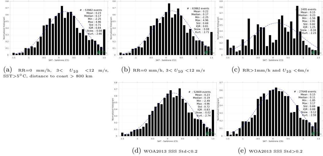
Figure 13: Normalized histogram of \Delta SSS (SMOS SSS L2Q v331 - With FLAG (CMEMS-CATDS-CPDC) - Saildrone) for 5 different subdatasets corresponding to: RR=0 mm/h, 3 < U_{10} < 12 m/s, SST>5°C, distance to coast > 800 km (a), RR=0 mm/h, 3 < U_{10} < 12 m/s (b), RR>1mm/h and U_{10} < 4 m/s (c), WOA2013 SSS Std<0.2 (d), WOA2013 SSS Std>0.2 (e).
