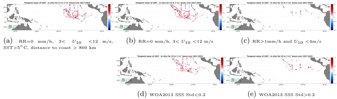
Figure 12: Temporal mean gridded over spatial boxes of size 1^\circ \times 1^\circ of \Delta SSS (SMOS SSS L2Q v331 - With FLAG (CMEMS-CATDS-CPDC) - Sairdrone) for 5 different subdatasets corresponding to: RR=0 mm/h, 3 < U_{10} < 12 m/s, SST > 5^\circ C , distance to coast > 800 km (a), RR=0 mm/h, 3 < U_{10} < 12 m/s (b), RR > 1 mm/h and U_{10} < 4 m/s (c), WOA2013 SSS Std < 0.2 (d), WOA2013 SSS Std > 0.2 (e).
