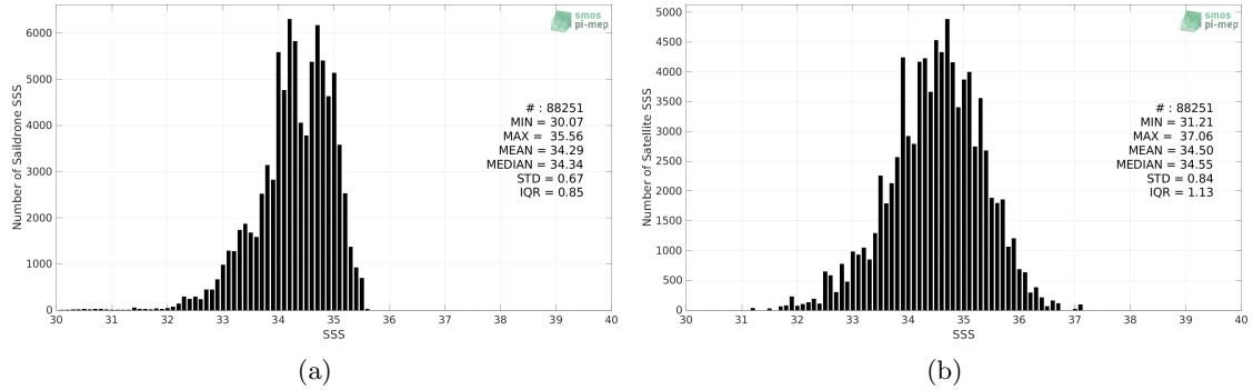
Figure 2: Histograms of SSS from Saildrone (a) and SMOS SSS L2Q v331 - With FLAG (CMEMS-CATDS-CPDC) (b) considering all match-up pairs per bins of 0.1 over the Tropical Pacific Ocean Pi-MEP region and for the full satellite product period.
