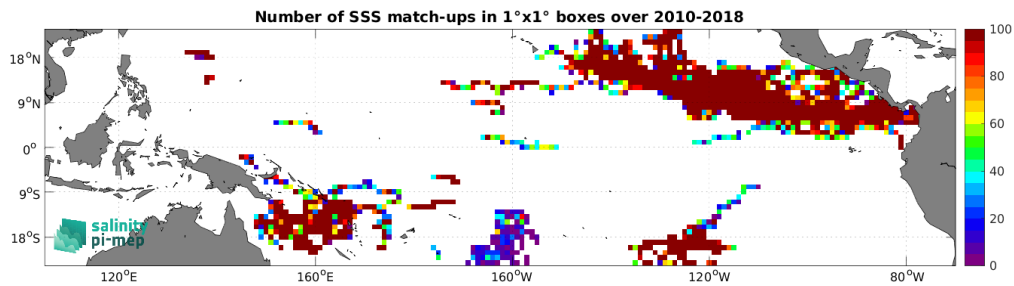
Figure 4: Number of SSS match-ups between Surface drifters SSS and the SMOS SSS L2Q v331 - With FLAG (CMEMS-CATDS-CPDC) SSS product for the Tropical Pacific Ocean Pi-MEP region over 1^\circ \times 1^\circ boxes and for the full satellite product period.
