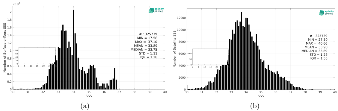
Figure 3: Histograms of SSS from Surface drifters (a) and SMOS SSS L2Q v331 - With FLAG (CMEMS-CATDS-CPDC) (b) considering all match-up pairs per bins of 0.1 over the Tropical Pacific Ocean Pi-MEP region and for the full satellite product period.
