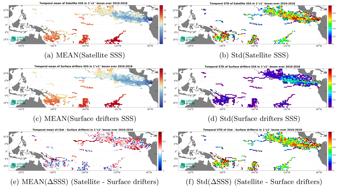
Figure 6: Temporal mean (left) and Std (right) of SSS from SMOS SSS L2Q v331 - With FLAG (CMEMS-CATDS-CPDC) (top), Surface drifters (middle), and of \Delta SSS (Satellite - Surface drifters). Only match-up pairs are used to generate these maps.
