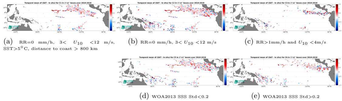
Figure 13: Temporal mean gridded over spatial boxes of size 1^\circ \times 1^\circ of \Delta SSS (SMOS SSS L2Q v331 - With FLAG (CMEMS-CATDS-CPDC) - Surface drifters) for 5 different subdatasets corresponding to: RR=0 mm/h, 3 < U_{10} < 12 m/s, SST > 5^\circ\text{C} , distance to coast > 800 km (a), RR=0 mm/h, 3 < U_{10} < 12 m/s (b), RR > 1 mm/h and U_{10} < 4 m/s (c), WOA2013 SSS Std < 0.2 (d), WOA2013 SSS Std > 0.2 (e).
