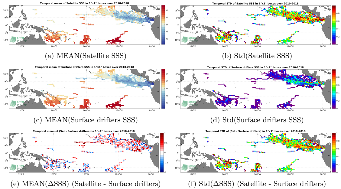
Figure 5: Temporal mean (left) and Std (right) of SSS from SMOS SSS L2Q v331 - With FLAG (CMEMS-CATDS-CPDC) (top), Surface drifters (middle), and of \Delta SSS (Satellite - Surface drifters). Only match-up pairs are used to generate these maps.
