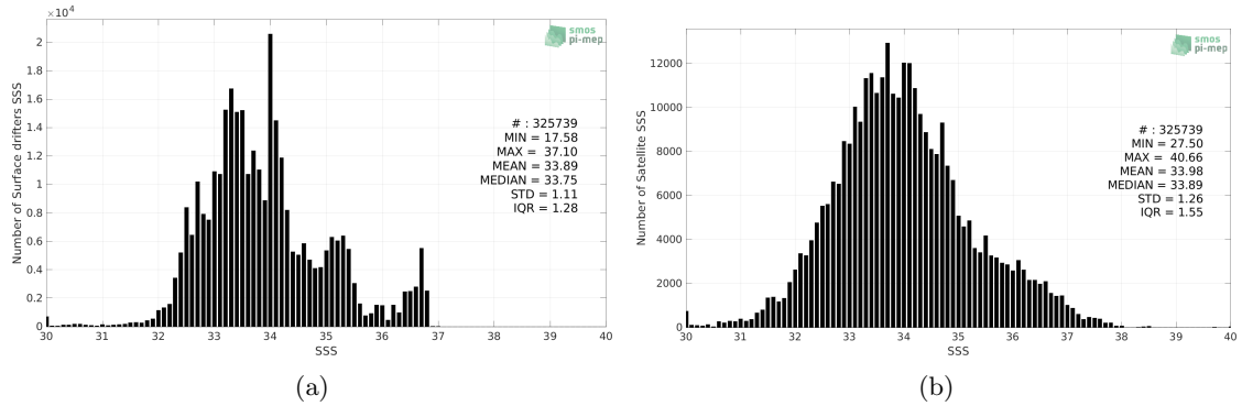
Figure 2: Histograms of SSS from Surface drifters (a) and SMOS SSS L2Q v331 - With FLAG (CMEMS-CATDS-CPDC) (b) considering all match-up pairs per bins of 0.1 over the Tropical Pacific Ocean Pi-MEP region and for the full satellite product period.
