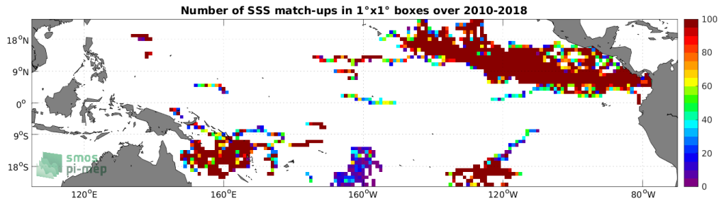
Figure 3: Number of SSS match-ups between Surface drifters SSS and the SMOS SSS L2Q v331 - With FLAG (CMEMS-CATDS-CPDC) SSS product for the Tropical Pacific Ocean Pi-MEP region over 1^\circ \times 1^\circ boxes and for the full satellite product period.
