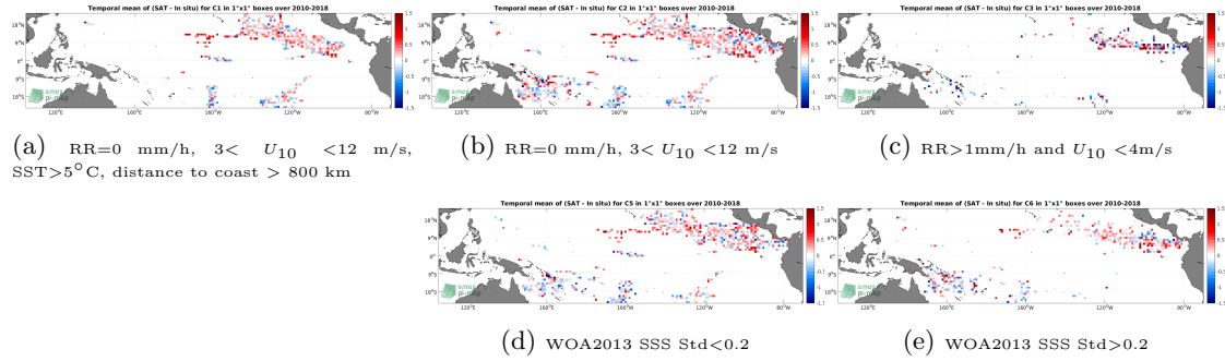
Figure 11: Temporal mean gridded over spatial boxes of size 1^{\circ}\times 1^{\circ} of \Delta\text{SSS} (SMOS SSS L2Q v331 - With FLAG (CMEMS-CATDS-CPDC) - Surface drifters) for 5 different subdatasets corresponding to: RR=0 mm/h, 3 < U_{10} < 12 m/s, SST > 5^{\circ}\text{C} , distance to coast > 800 km (a), RR=0 mm/h, 3 < U_{10} < 12 m/s (b), RR > 1 mm/h and U_{10} < 4 m/s (c), WOA2013 SSS Std < 0.2 (d), WOA2013 SSS Std > 0.2 (e).
