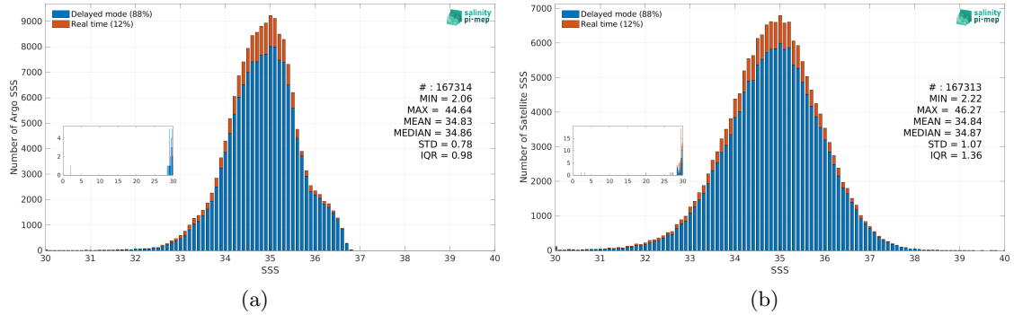
Figure 3: Histograms of SSS from Argo (a) and SMOS SSS L2Q v331 - With FLAG (CMEMS-CATDS-CPDC) (b) considering all match-up pairs per bins of 0.1 over the Tropical Pacific Ocean Pi-MEP region and for the full satellite product period.
