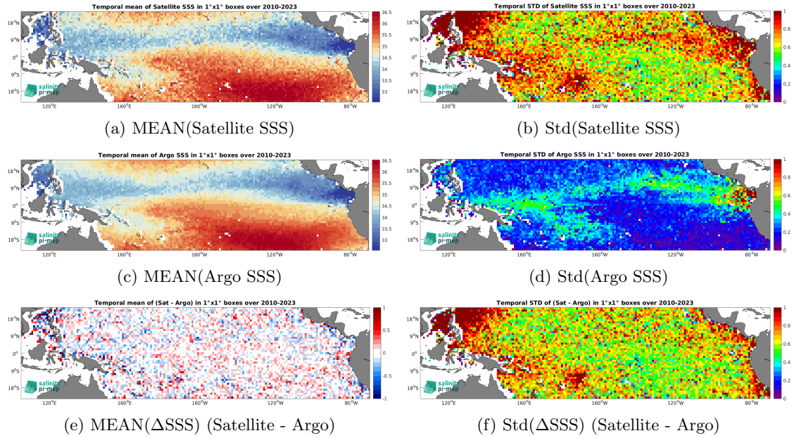
Figure 6: Temporal mean (left) and Std (right) of SSS from SMOS SSS L2Q v331 - With FLAG (CMEMS-CATDS-CPDC) (top), Argo (middle), and of \Delta SSS (Satellite - Argo). Only match-up pairs are used to generate these maps.
