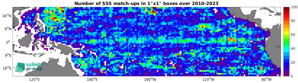
Figure 4: Number of SSS match-ups between Argo SSS and the SMOS SSS L2Q v331 - With FLAG (CMEMS-CATDS-CPDC) SSS product for the Tropical Pacific Ocean Pi-MEP region over 1^\circ \times 1^\circ boxes and for the full satellite product period.
