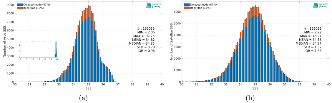
Figure 2: Histograms of SSS from Argo (a) and SMOS SSS L2Q v331 - With FLAG (CMEMS-CATDS-CPDC) (b) considering all match-up pairs per bins of 0.1 over the Tropical Pacific Ocean Pi-MEP region and for the full satellite product period.
