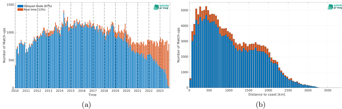
Figure 1: Number of match-ups between Argo and SMOS SSS L2Q v331 - With FLAG (CMEMS-CATDS-CPDC) SSS as a function of time (a) and as function of the distance to coast (b) over the Tropical Pacific Ocean Pi-MEP region and for the full satellite product period.
