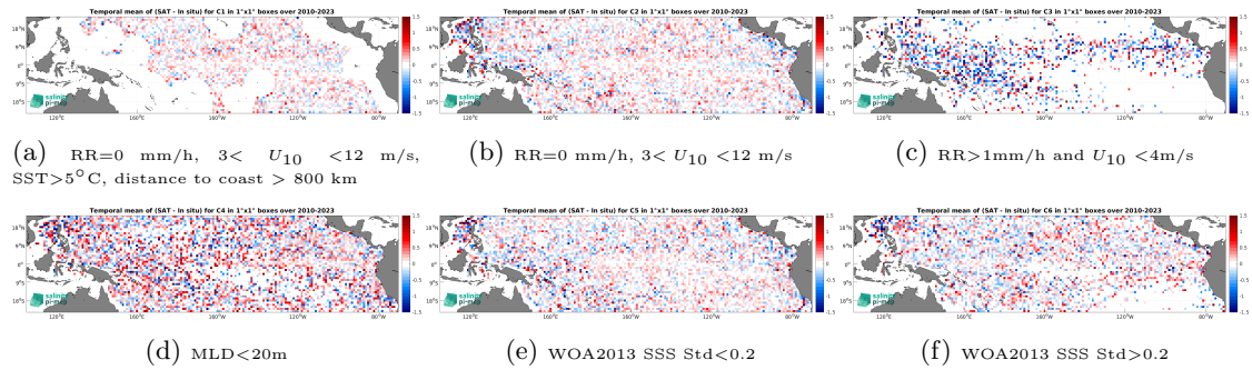
Figure 12: Temporal mean gridded over spatial boxes of size 1^\circ \times 1^\circ of \Delta SSS (SMOS SSS L2Q v331 - With FLAG (CMEMS-CATDS-CPDC) - Argo) for 6 different subdatasets corresponding to:RR=0 mm/h, 3 < U_{10} < 12 m/s, SST >5^\circ\text{C} , distance to coast > 800 km (a), RR=0 mm/h, 3 < U_{10} < 12 m/s (b), RR >1 mm/h and U_{10} < 4 m/s (c),MLD <20 m (d),WOA2013 SSS Std <0.2 (e),WOA2013 SSS Std >0.2 (f).
