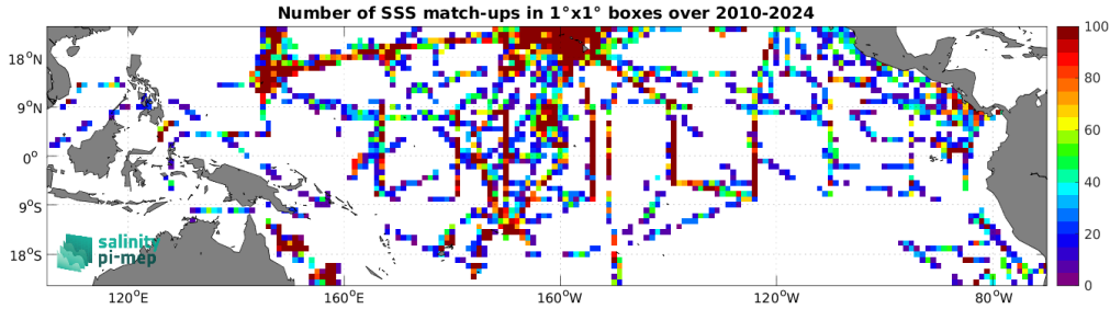
Figure 5: Number of SSS match-ups between TSG (SAMOS) SSS and the SMOS SSS L2Q v331 - No FLAG (CMEMS-CATDS-CPDC) SSS product for the Tropical Pacific Ocean Pi-MEP region over 1^\circ \times 1^\circ boxes and for the full satellite product period.
