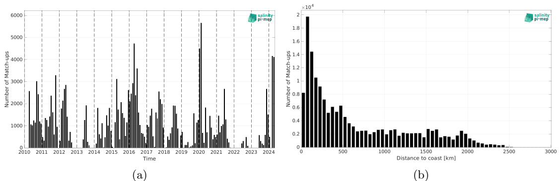
Figure 2: Number of match-ups between TSG (SAMOS) and SMOS SSS L2Q v331 - No FLAG (CMEMS-CATDS-CPDC) SSS as a function of time (a) and as function of the distance to coast (b) over the Tropical Pacific Ocean Pi-MEP region and for the full satellite product period.
