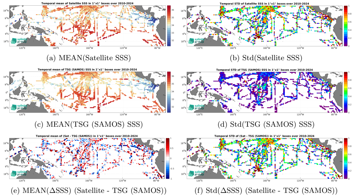
Figure 7: Temporal mean (left) and Std (right) of SSS from SMOS SSS L2Q v331 - No FLAG (CMEMS-CATDS-CPDC) (top), TSG (SAMOS) (middle), and of \Delta SSS (Satellite - TSG (SAMOS)). Only match-up pairs are used to generate these maps.
