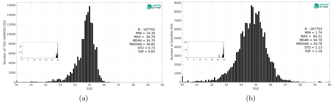
Figure 3: Histograms of SSS from TSG (SAMOS) (a) and SMOS SSS L2Q v331 - No FLAG (CMEMS-CATDS-CPDC) (b) considering all match-up pairs per bins of 0.1 over the Tropical Pacific Ocean Pi-MEP region and for the full satellite product period.
