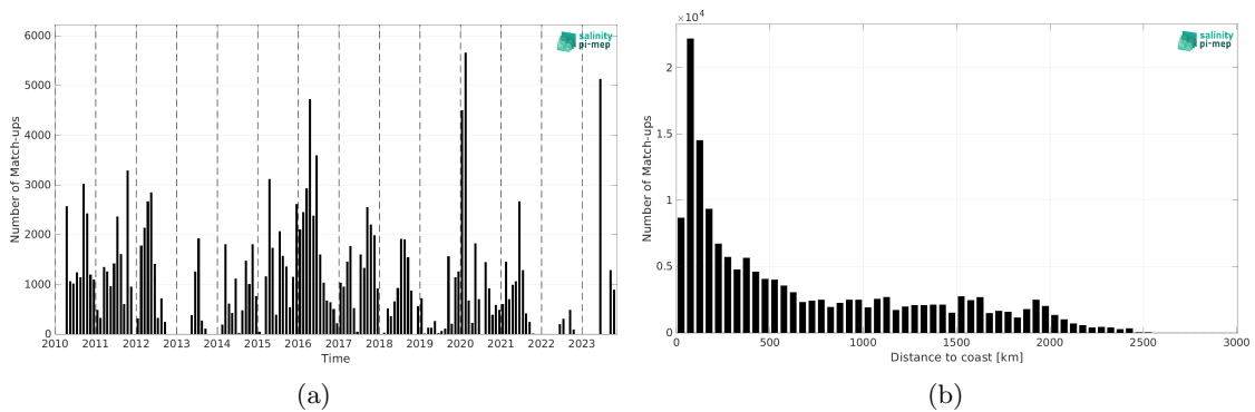
Figure 1: Number of match-ups between TSG (SAMOS) and SMOS SSS L2Q v331 - No FLAG (CMEMS-CATDS-CPDC) SSS as a function of time (a) and as function of the distance to coast (b) over the Tropical Pacific Ocean Pi-MEP region and for the full satellite product period.
