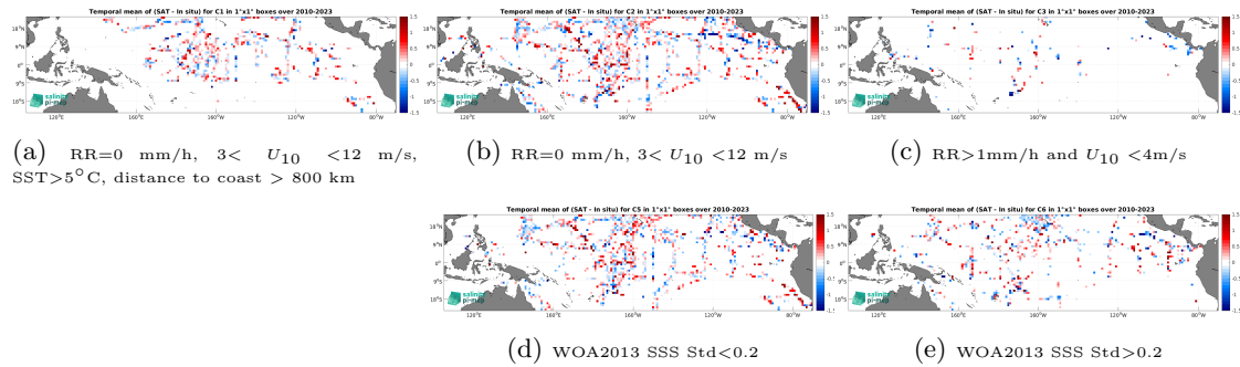
Figure 12: Temporal mean gridded over spatial boxes of size 1^{\circ}\times 1^{\circ} of \Delta\text{SSS} (SMOS SSS L2Q v331 - No FLAG (CMEMS-CATDS-CPDC) - TSG (SAMOS)) for 5 different subdatasets corresponding to:RR=0 mm/h, 3 < U_{10} < 12 m/s, SST >5^{\circ}\text{C} , distance to coast > 800 km (a), RR=0 mm/h, 3 < U_{10} < 12 m/s (b), RR >1 mm/h and U_{10} < 4 m/s (c), WOA2013 SSS Std <0.2 (d), WOA2013 SSS Std >0.2 (e).
