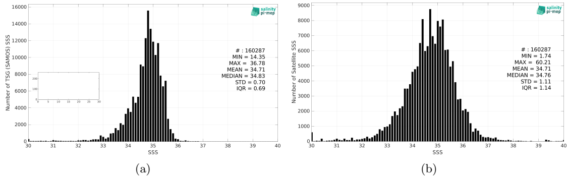
Figure 2: Histograms of SSS from TSG (SAMOS) (a) and SMOS SSS L2Q v331 - No FLAG (CMEMS-CATDS-CPDC) (b) considering all match-up pairs per bins of 0.1 over the Tropical Pacific Ocean Pi-MEP region and for the full satellite product period.
