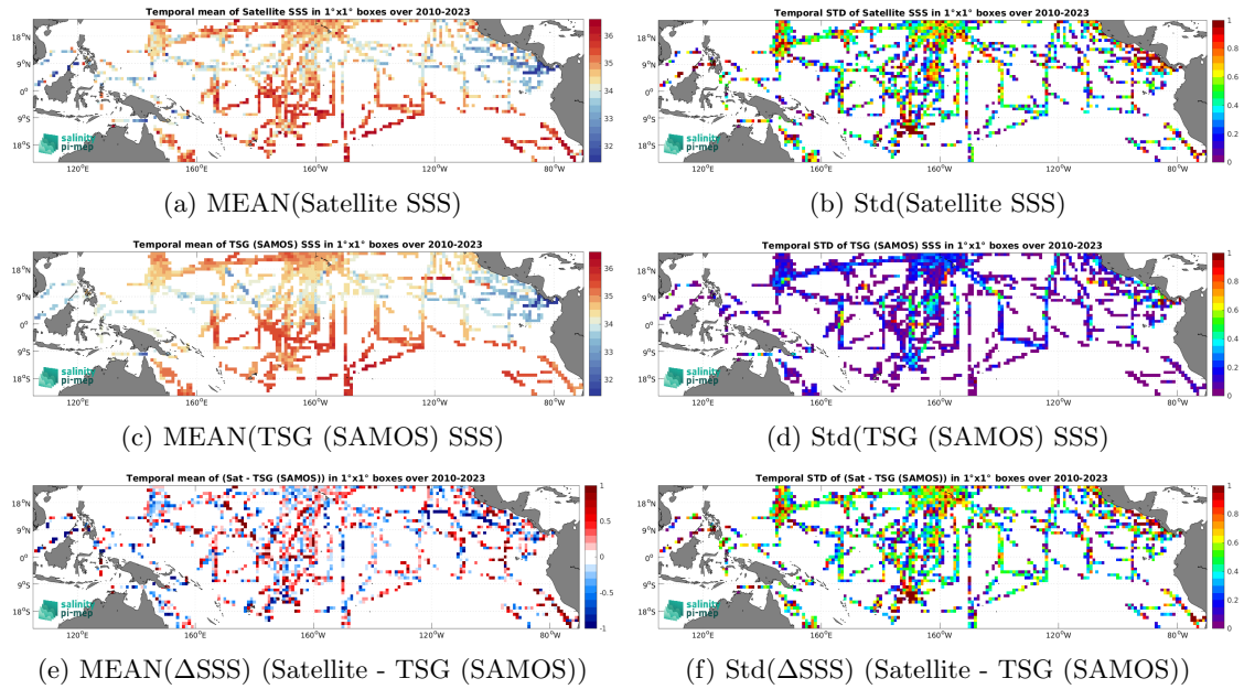
Figure 6: Temporal mean (left) and Std (right) of SSS from SMOS SSS L2Q v331 - No FLAG (CMEMS-CATDS-CPDC) (top), TSG (SAMOS) (middle), and of \Delta SSS (Satellite - TSG (SAMOS)). Only match-up pairs are used to generate these maps.
