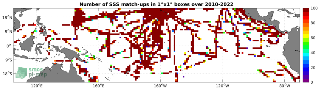
Figure 4: Number of SSS match-ups between TSG (SAMOS) SSS and the SMOS SSS L2Q v331 - No FLAG (CMEMS-CATDS-CPDC) SSS product for the Tropical Pacific Ocean Pi-MEP region over 1^\circ \times 1^\circ boxes and for the full satellite product period.
