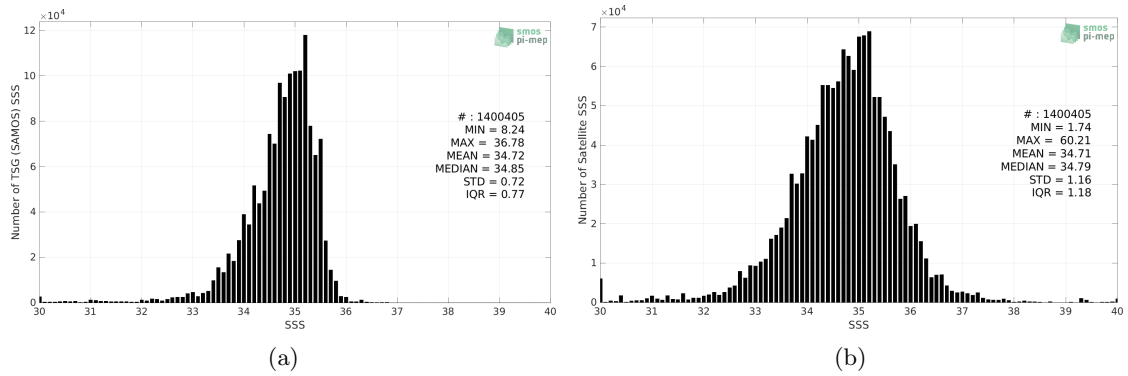
Figure 2: Histograms of SSS from TSG (SAMOS) (a) and SMOS SSS L2Q v331 - No FLAG (CMEMS-CATDS-CPDC) (b) considering all match-up pairs per bins of 0.1 over the Tropical Pacific Ocean Pi-MEP region and for the full satellite product period.
