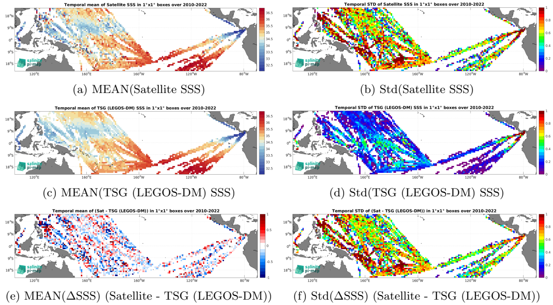
Figure 7: Temporal mean (left) and Std (right) of SSS from SMOS SSS L2Q v331 - No FLAG (CMEMS-CATDS-CPDC) (top), TSG (LEGOS-DM) (middle), and of \Delta SSS (Satellite - TSG (LEGOS-DM)). Only match-up pairs are used to generate these maps.
