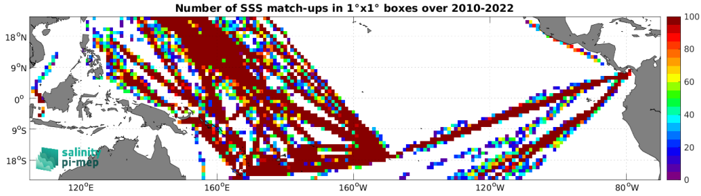
Figure 5: Number of SSS match-ups between TSG (LEGOS-DM) SSS and the SMOS SSS L2Q v331 - No FLAG (CMEMS-CATDS-CPDC) SSS product for the Tropical Pacific Ocean Pi-MEP region over 1^\circ \times 1^\circ boxes and for the full satellite product period.
