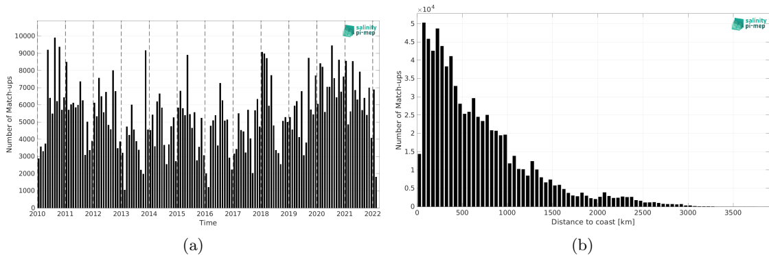
Figure 2: Number of match-ups between TSG (LEGOS-DM) and SMOS SSS L2Q v331 - No FLAG (CMEMS-CATDS-CPDC) SSS as a function of time (a) and as function of the distance to coast (b) over the Tropical Pacific Ocean Pi-MEP region and for the full satellite product period.
