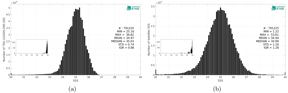
Figure 3: Histograms of SSS from TSG (LEGOS-DM) (a) and SMOS SSS L2Q v331 - No FLAG (CMEMS-CATDS-CPDC) (b) considering all match-up pairs per bins of 0.1 over the Tropical Pacific Ocean Pi-MEP region and for the full satellite product period.
