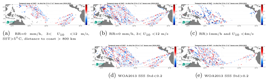
Figure 14: Temporal mean gridded over spatial boxes of size 1^\circ \times 1^\circ of \Delta SSS (SMOS SSS L2Q v331 - No FLAG (CMEMS-CATDS-CPDC) - TSG (LEGOS-DM)) for 5 different subdatasets corresponding to:RR=0 mm/h, 3 < U_{10} < 12 m/s, SST > 5^\circ\text{C} , distance to coast > 800 km (a), RR=0 mm/h, 3 < U_{10} < 12 m/s (b), RR > 1 mm/h and U_{10} < 4 m/s (c), WOA2013 SSS Std < 0.2 (d), WOA2013 SSS Std > 0.2 (e).
