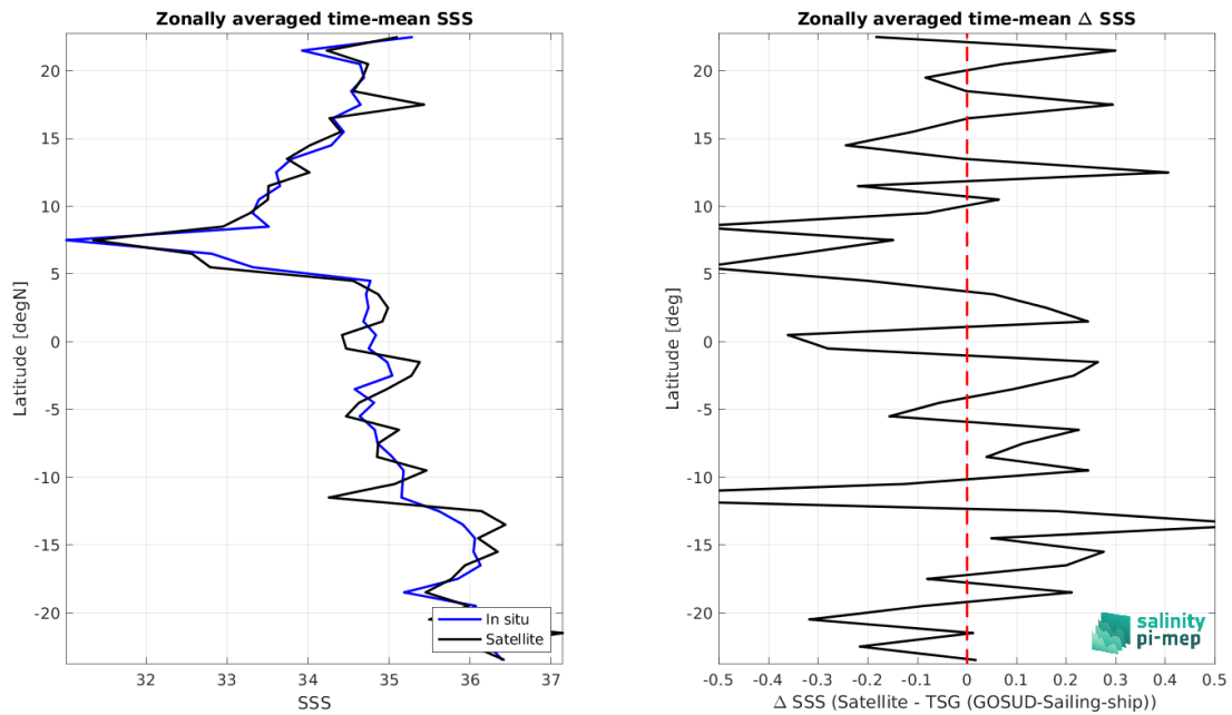
Figure 9: Left panel: Zonal mean SSS from SMOS SSS L2Q v331 - No FLAG (CMEMS-CATDS-CPDC) satellite product (black) and from TSG (GOSUD-Sailing-ship) (blue). Right panel: Zonal mean of \Delta SSS (Satellite - TSG (GOSUD-Sailing-ship)) for all the collected Pi-MEP match-up pairs estimated over the full satellite product period.
