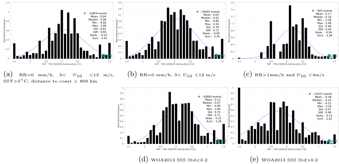
Figure 15: Normalized histogram of \Delta\text{SSS} (SMOS SSS L2Q v331 - No FLAG (CMEMS-CATDS-CPDC) - TSG (GOSUD-Sailing-ship)) for 5 different subdatasets corresponding to: RR=0 mm/h, 3 < U_{10} < 12 m/s, SST > 5^\circ\text{C} , distance to coast > 800 km (a), RR=0 mm/h, 3 < U_{10} < 12 m/s (b), RR > 1 mm/h and U_{10} < 4 m/s (c), WOA2013 SSS Std < 0.2 (d), WOA2013 SSS Std > 0.2 (e).
