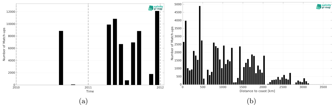
Figure 2: Number of match-ups between TSG (GOSUD-Sailing-ship) and SMOS SSS L2Q v331 - No FLAG (CMEMS-CATDS-CPDC) SSS as a function of time (a) and as function of the distance to coast (b) over the Tropical Pacific Ocean Pi-MEP region and for the full satellite product period.
