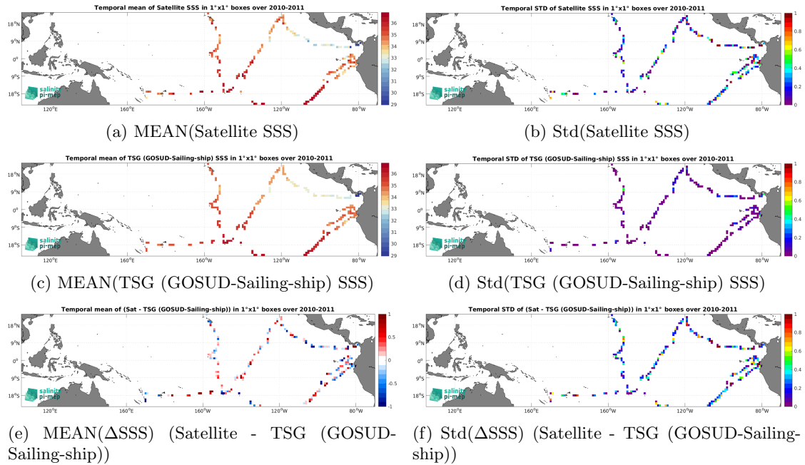
Figure 7: Temporal mean (left) and Std (right) of SSS from SMOS SSS L2Q v331 - No FLAG (CMEMS-CATDS-CPDC) (top), TSG (GOSUD-Sailing-ship) (middle), and of \Delta SSS (Satellite - TSG (GOSUD-Sailing-ship)). Only match-up pairs are used to generate these maps.
