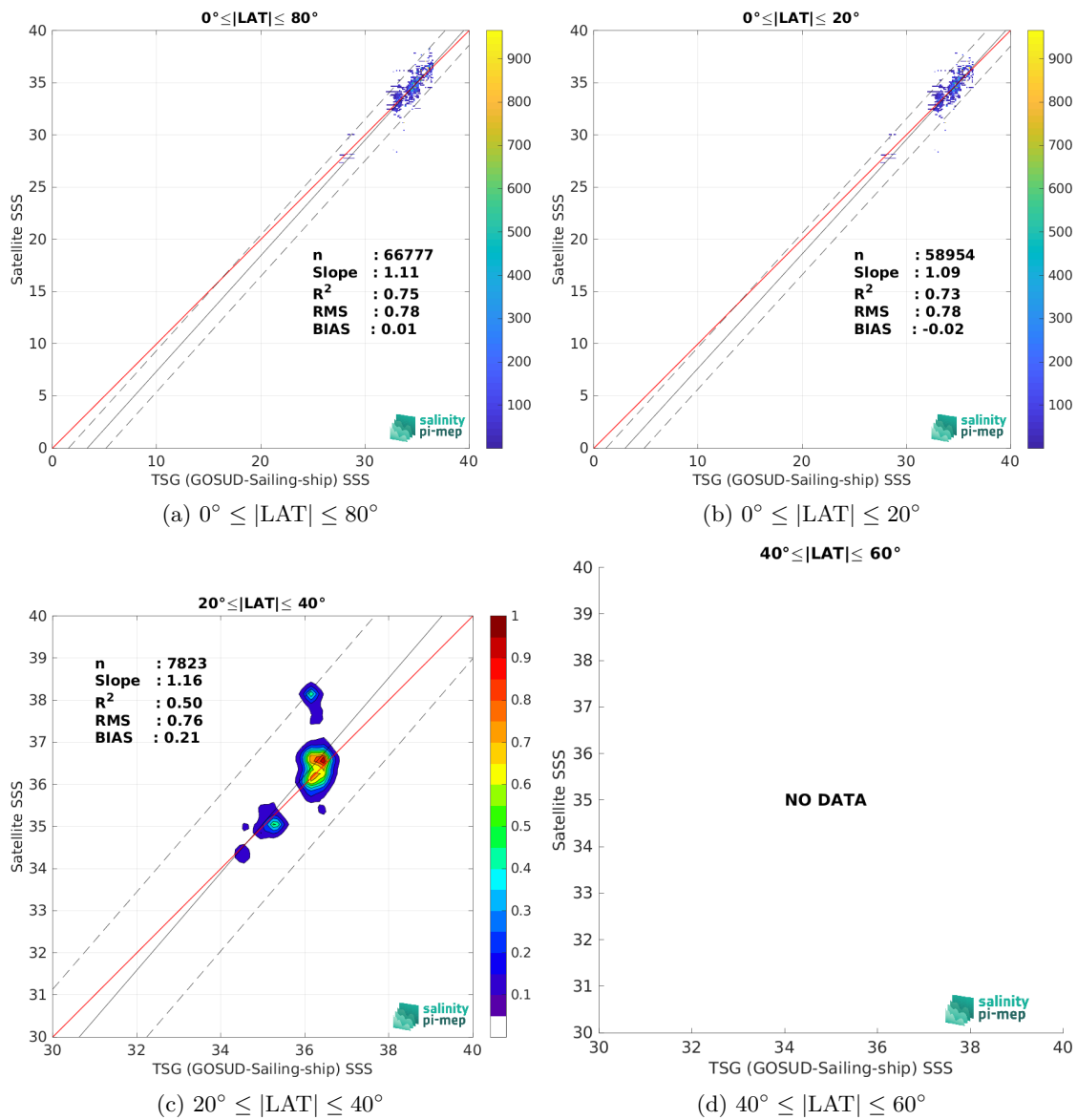
Figure 10: Contour maps of the concentration of SMOS SSS L2Q v331 - No FLAG (CMEMS-CATDS-CPDC) SSS (y-axis) versus TSG (GOSUD-Sailing-ship) SSS (x-axis) at match-up pairs for different latitude bands. For each plot, the red line shows x=y . The black thin and dashed lines indicate a linear fit through the data cloud and the \pm 95\% confidence levels, respectively. The number match-up pairs n , the slope and R^2 coefficient of the linear fit, the root mean square (RMS) and the mean bias between satellite and in situ data are indicated for each latitude band in each plots.
