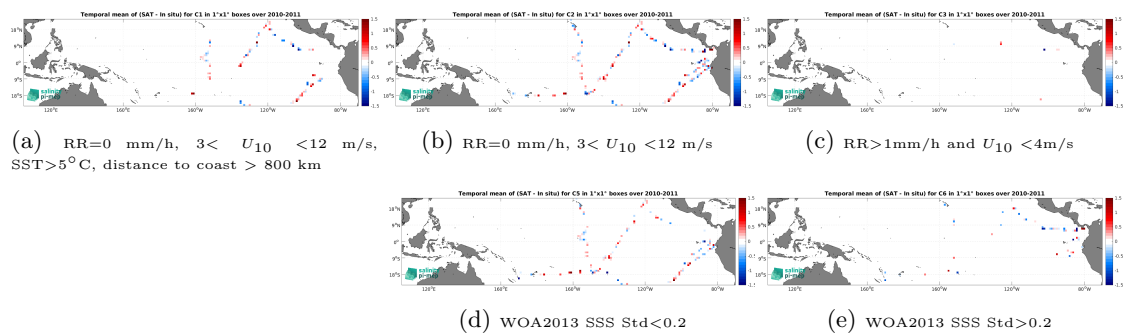
Figure 14: Temporal mean gridded over spatial boxes of size 1^\circ \times 1^\circ of \Delta SSS (SMOS SSS L2Q v331 - No FLAG (CMEMS-CATDS-CPDC) - TSG (GOSUD-Sailing-ship)) for 5 different sub-datasets corresponding to: RR=0 mm/h, 3 < U_{10} < 12 m/s, SST > 5^\circ\text{C} , distance to coast > 800 km (a), RR=0 mm/h, 3 < U_{10} < 12 m/s (b), RR > 1 mm/h and U_{10} < 4 m/s (c), WOA2013 SSS Std < 0.2 (d), WOA2013 SSS Std > 0.2 (e).
