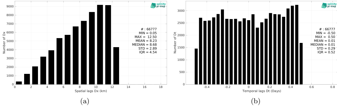
Figure 6: Histograms of the spatial (a) and temporal (b) lags between the location/time of the TSG (GOSUD-Sailing-ship) measurement and the date of the corresponding SMOS SSS L2Q v331 - No FLAG (CMEMS-CATDS-CPDC) SSS pixel.
