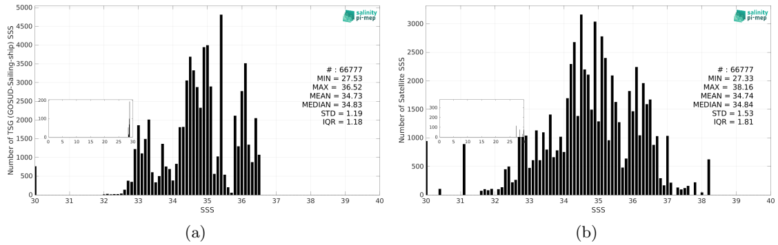
Figure 3: Histograms of SSS from TSG (GOSUD-Sailing-ship) (a) and SMOS SSS L2Q v331 - No FLAG (CMEMS-CATDS-CPDC) (b) considering all match-up pairs per bins of 0.1 over the Tropical Pacific Ocean Pi-MEP region and for the full satellite product period.
